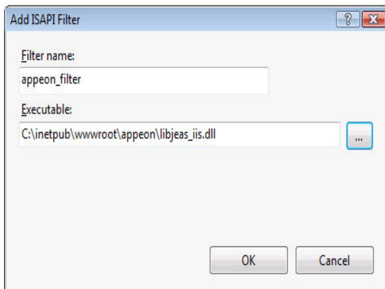
Figure 2.11: Add ISAPI filter
