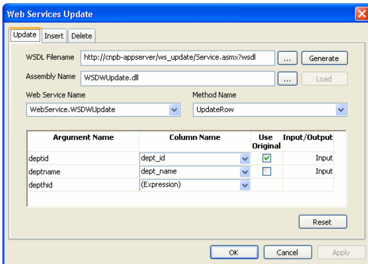
Figure 21.6: Web Service Update dialog box
