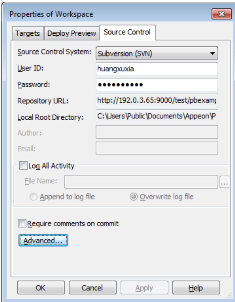
Figure 3.7: Source Control
