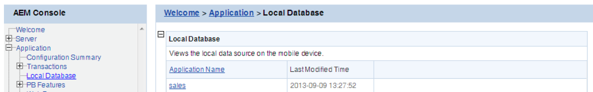
Figure 5.67: Local database
