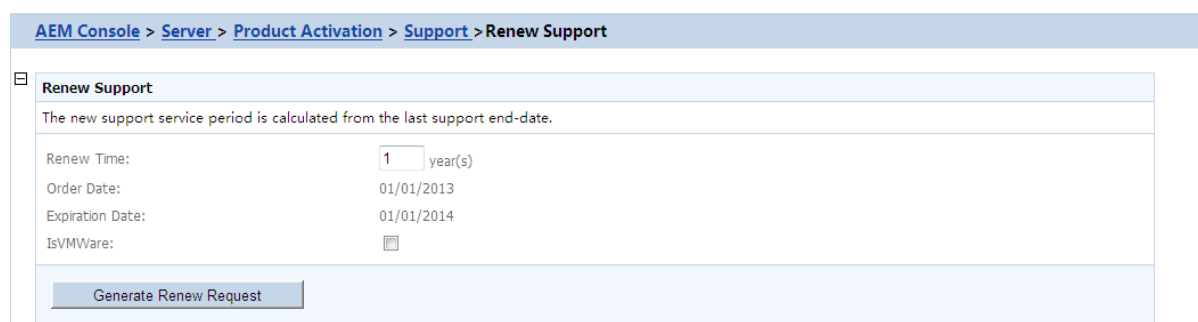
Figure 5.39: Renew support
