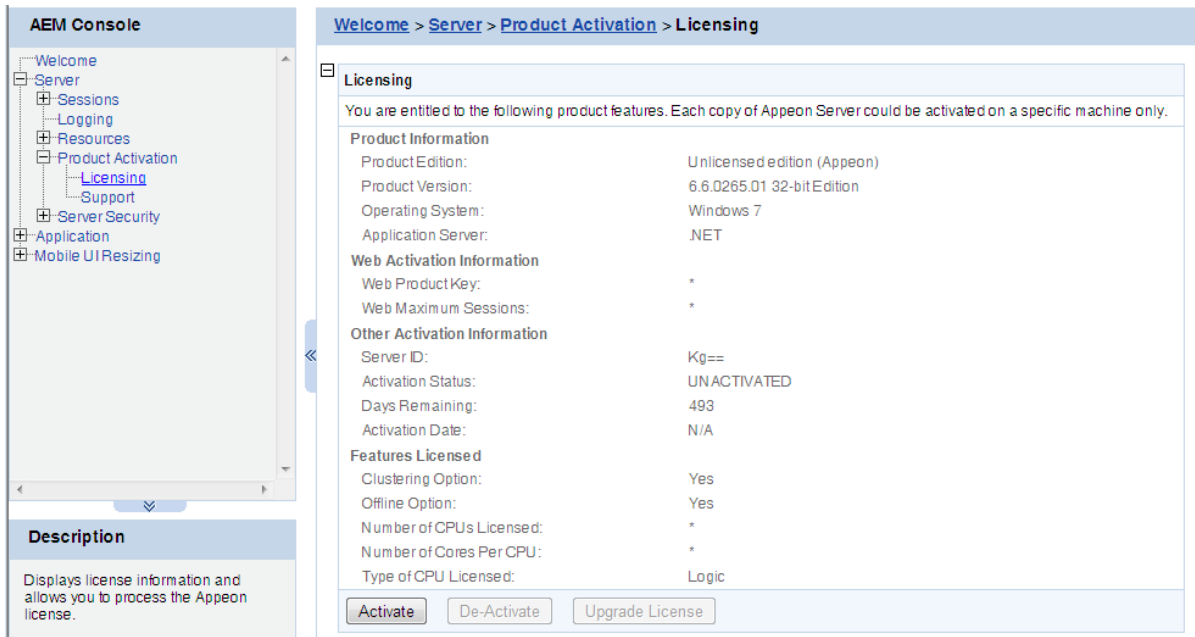
Figure 5.24: Licensing
