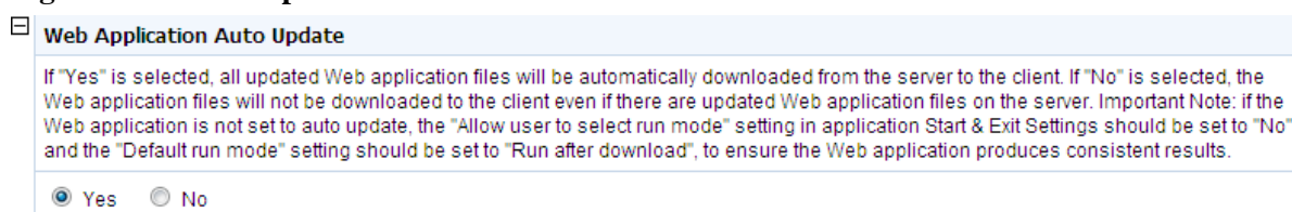
Figure 5.89: Auto Update
