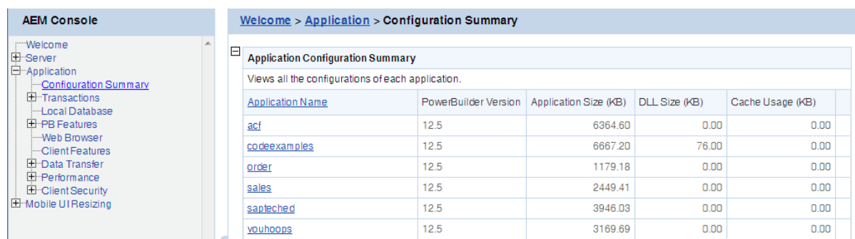
Figure 5.59: Application Summary
