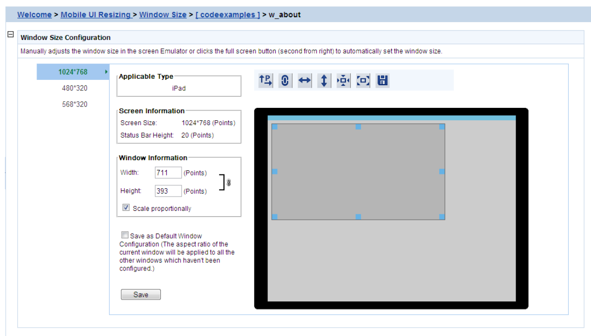
Figure 5.125: Screen emulator
