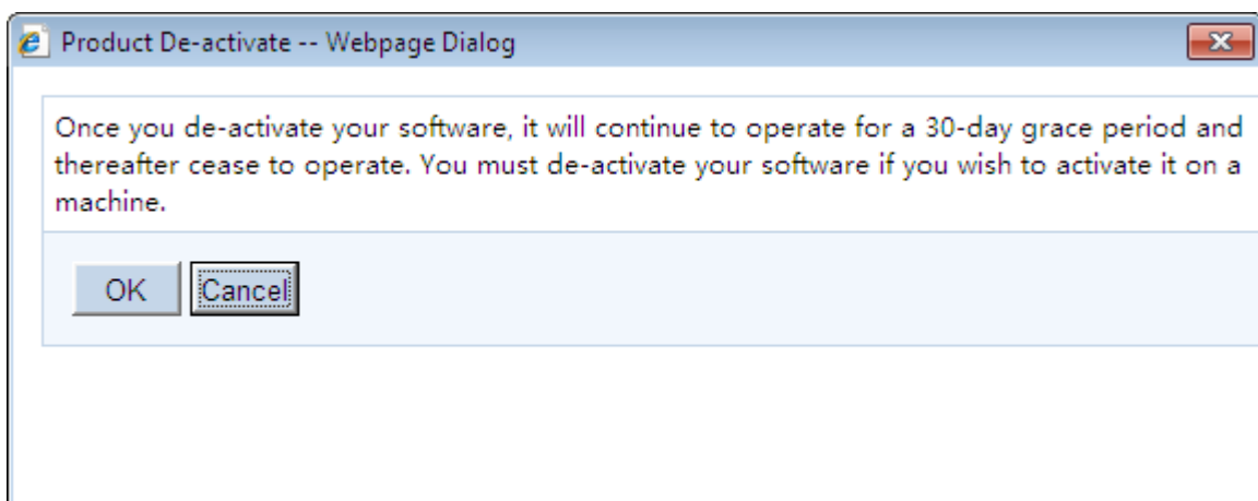
Figure 5.32: Product De-activate
