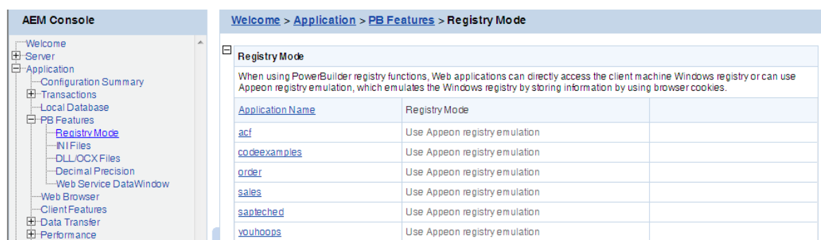
Figure 5.70: Registry Mode
