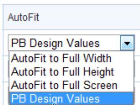
Figure 5.123: Autofit mode
