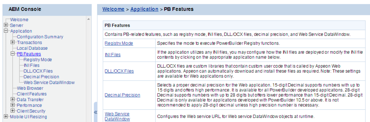
Figure 5.69: PB Features
