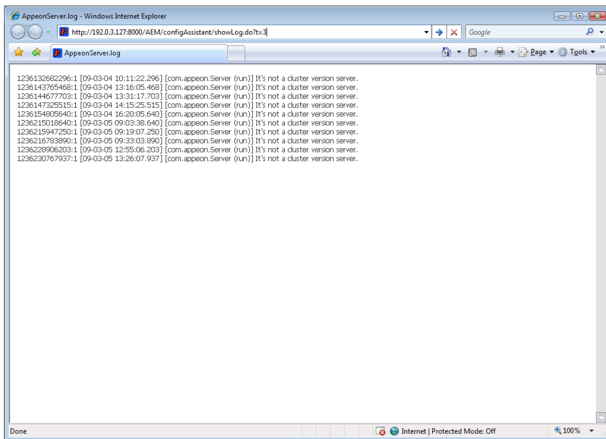
Figure 5.13: Deployment Log
