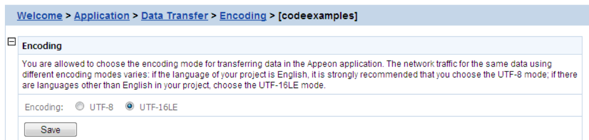
Figure 5.102: Encoding settings
