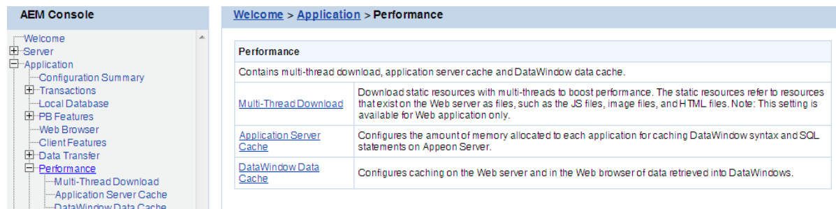
Figure 5.103: Performance
