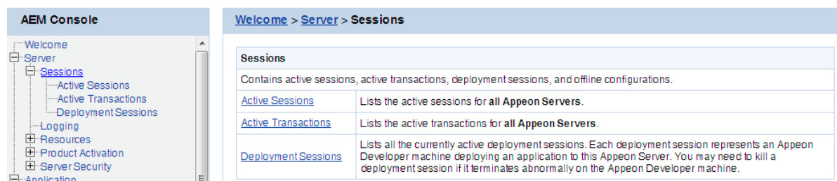
Figure 5.8: Sessions
