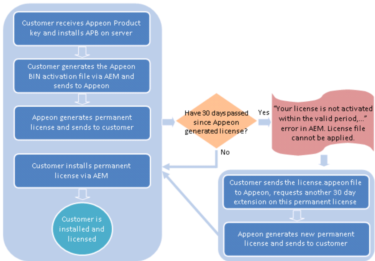
Figure 5.25: Activation process
