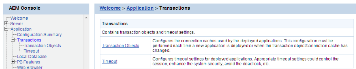
Figure 5.61: Transactions
