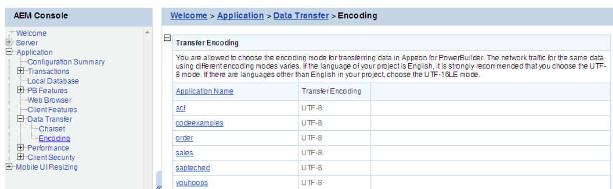
Figure 5.101: Encoding
