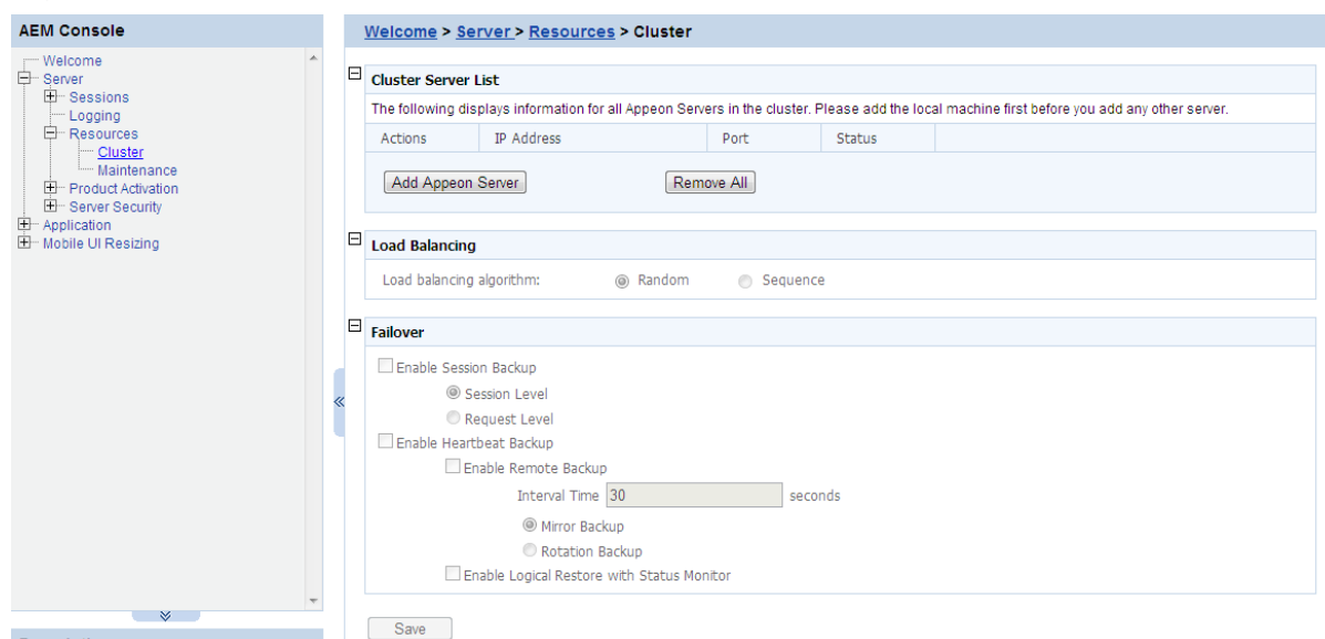
Figure 5.16: Cluster
