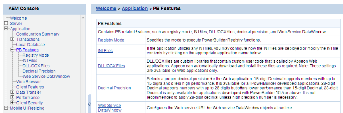
Figure 5.70: PB Features
