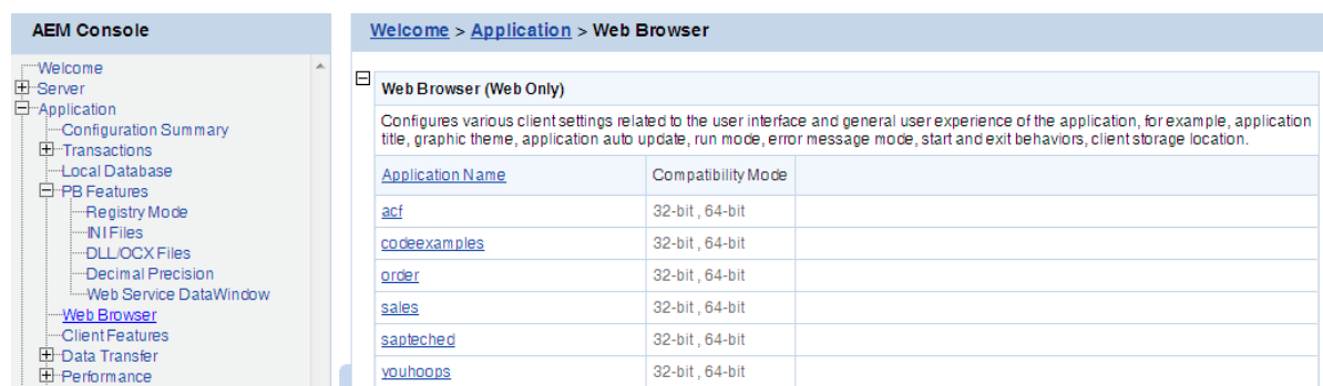
Figure 5.84: Web Browser
