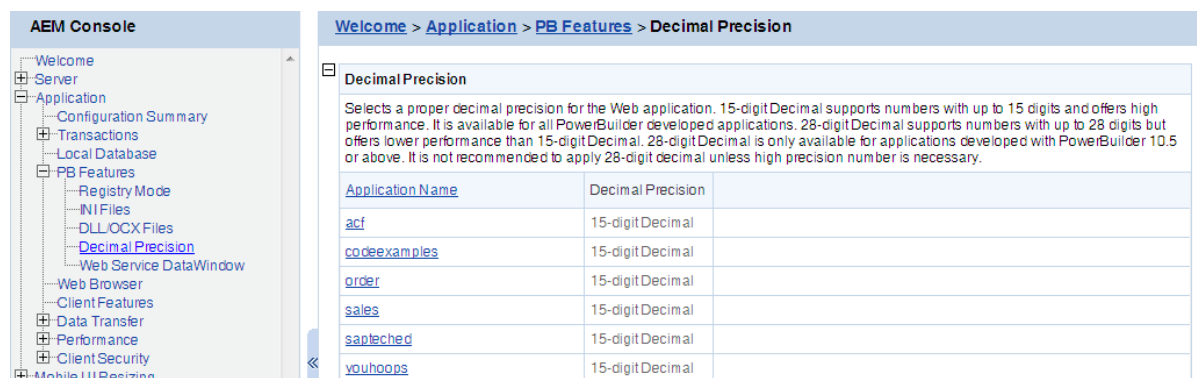
Figure 5.79: Decimal Precision
