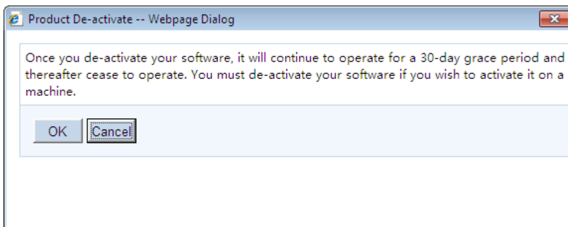
Figure 5.33: Product De-activate
