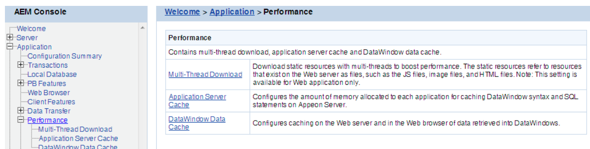
Figure 5.104: Performance
