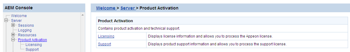
Figure 5.24: Product Activation
