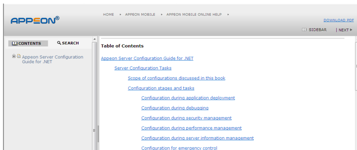
Figure 5.7: Apeon Help
