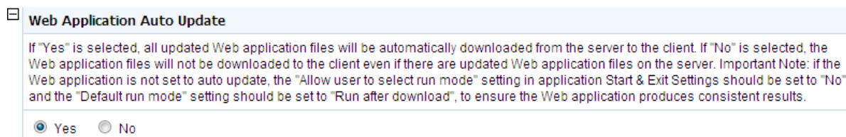
Figure 5.90: Auto Update
