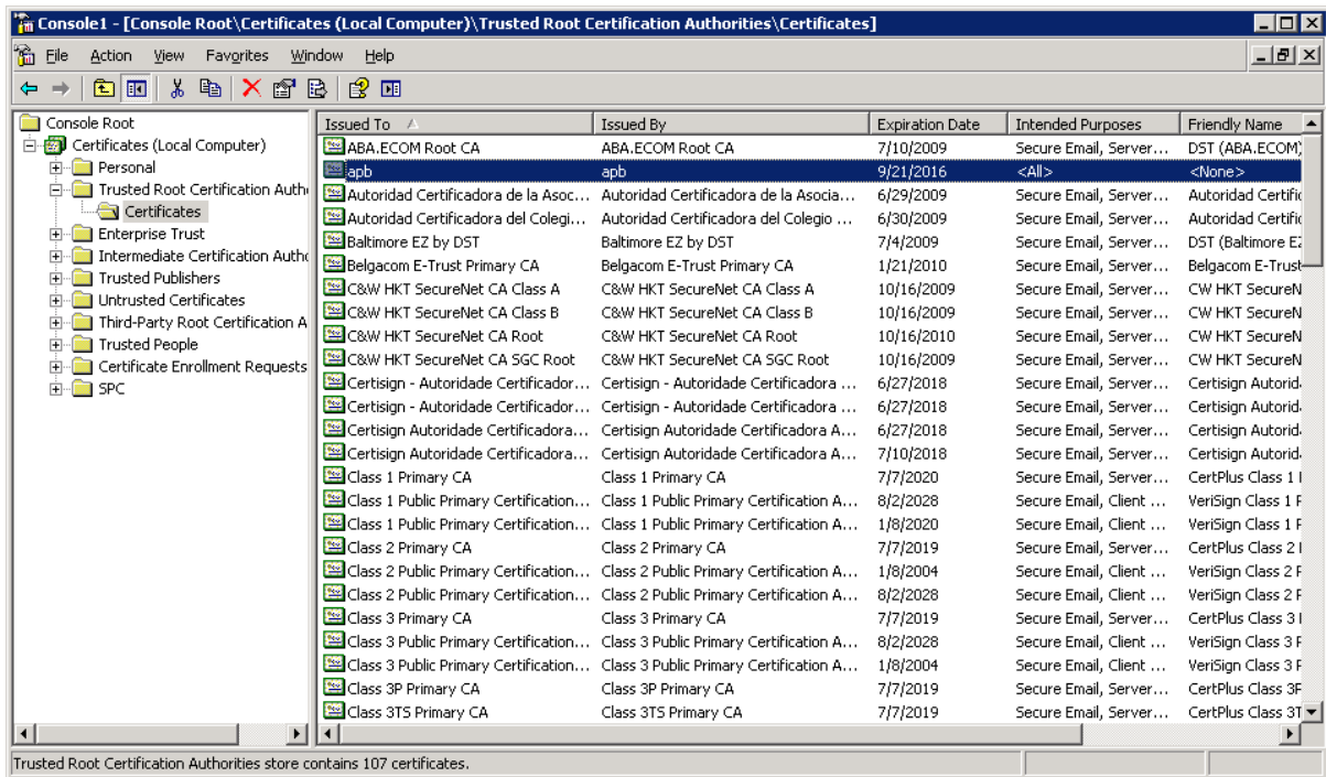
Figure 5.57: Imported Certificates
