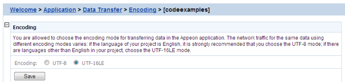
Figure 5.103: Encoding settings
