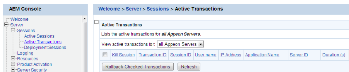
Figure 5.11: Active Transactions
