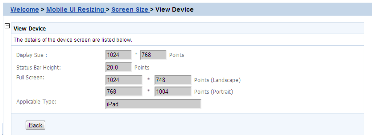
Figure 5.119: Screen details
