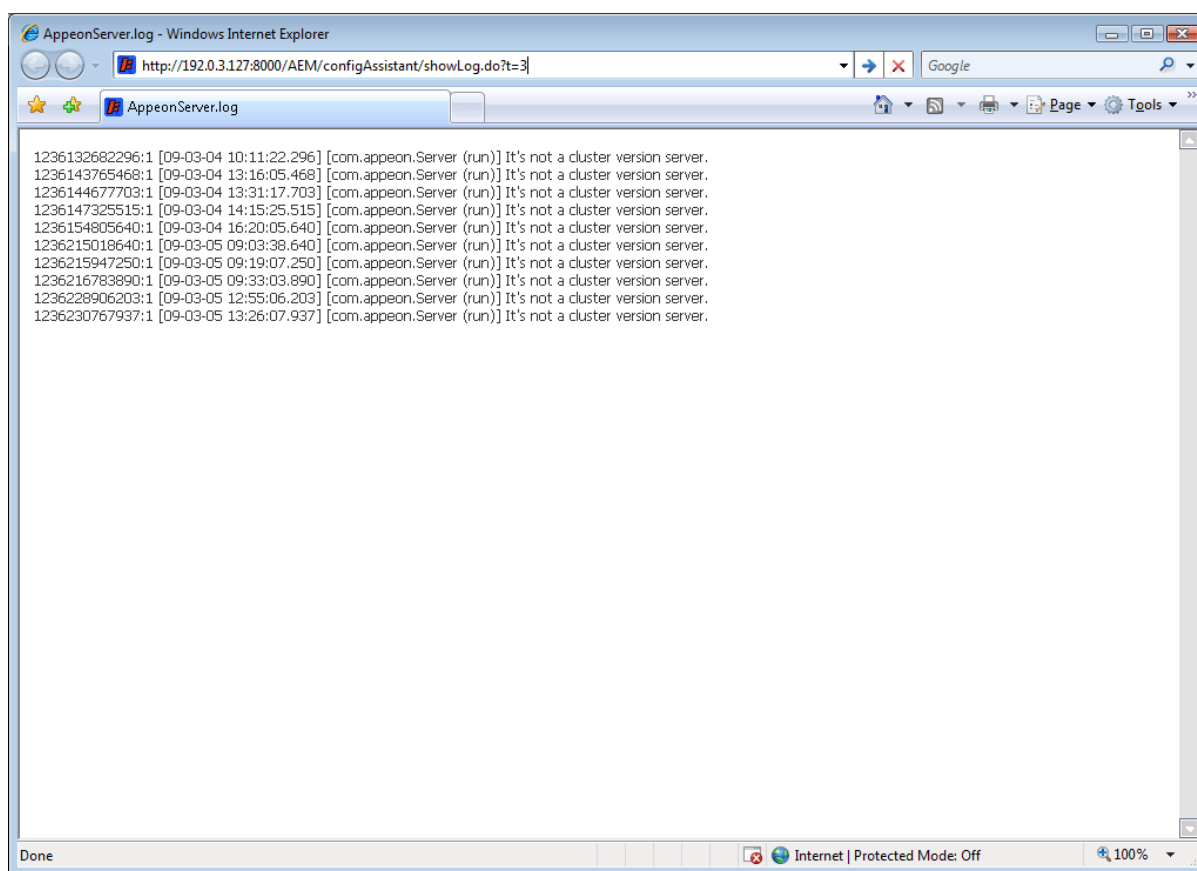
Figure 5.14: Deployment Log
