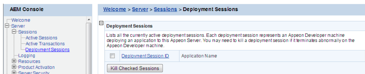
Figure 5.12: Deployment Sessions
