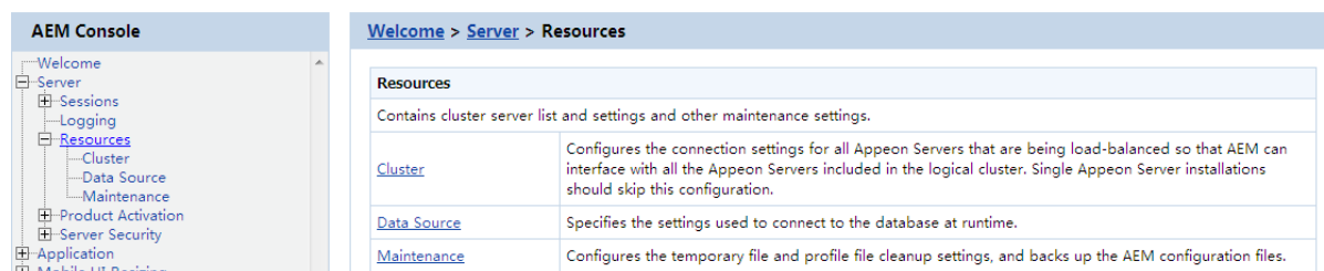
Figure 5.15: Resources
