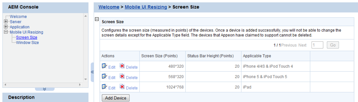
Figure 5.118: Screen Size
