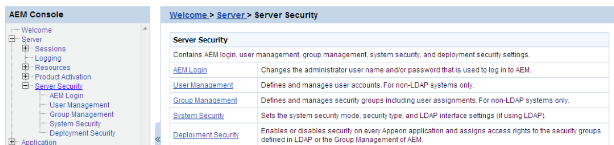
Figure 5.44: Server Security
