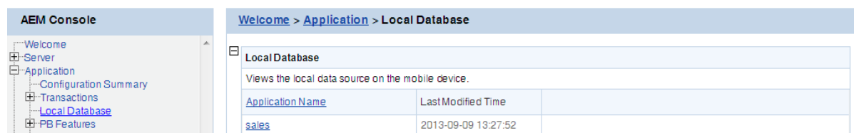
Figure 5.68: Local database
