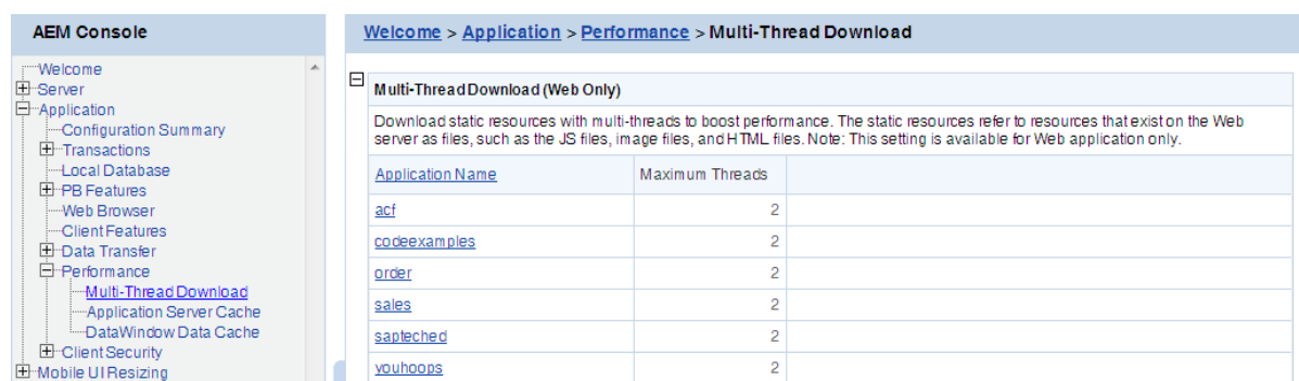
Figure 5.105: Multi-thread Download
