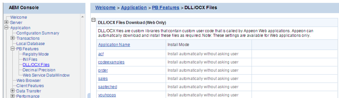
Figure 5.77: DLL/OCX Files
