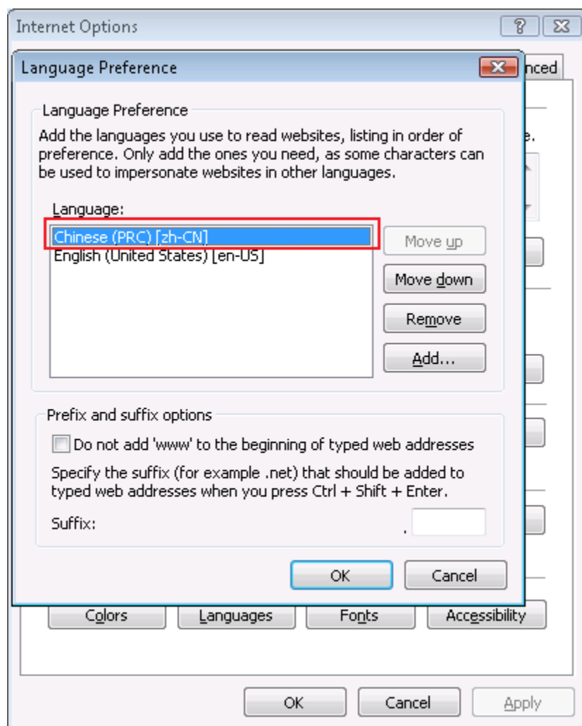
Figure 5.5: Language settings
