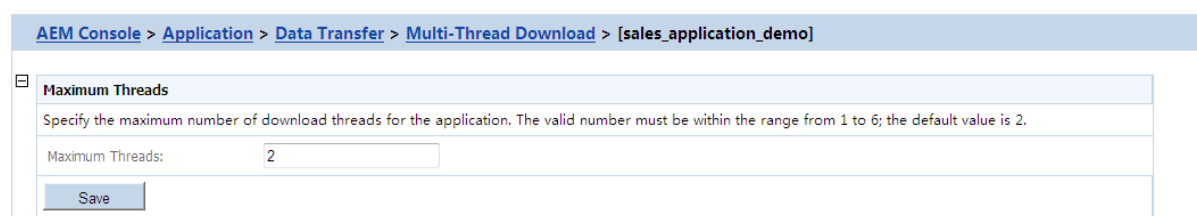
Figure 5.106: Maximum Threads
