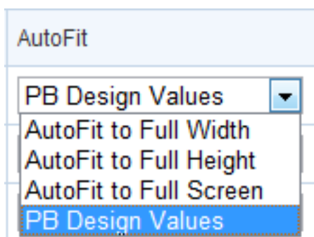
Figure 5.124: Autofit mode
