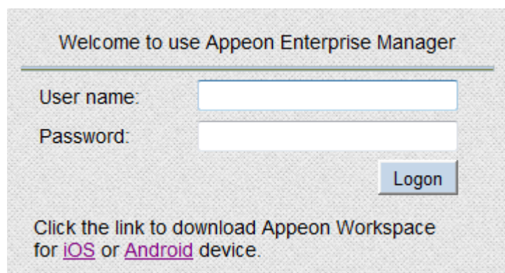
Figure 5.3: AEM login
