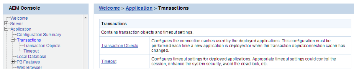
Figure 5.62: Transactions
