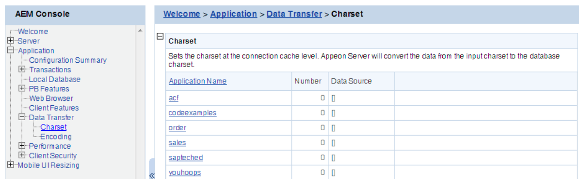
Figure 5.99: Charset settings
