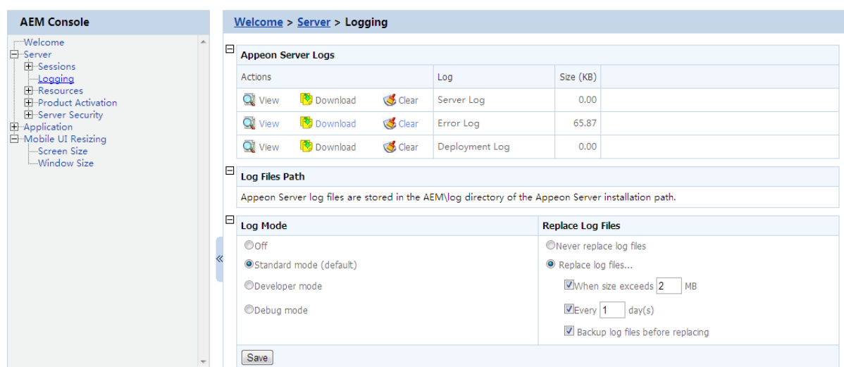
Figure 5.13: Logging
