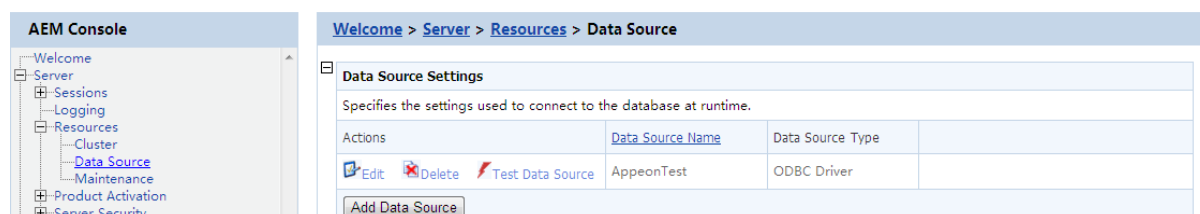
Figure 5.18: Data source
