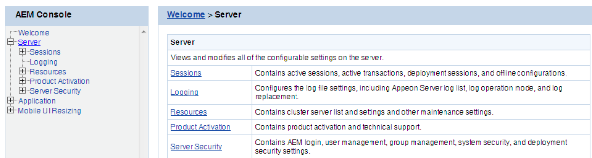
Figure 5.8: Server
