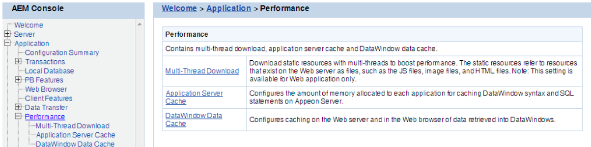
Figure 5.97: Performance
