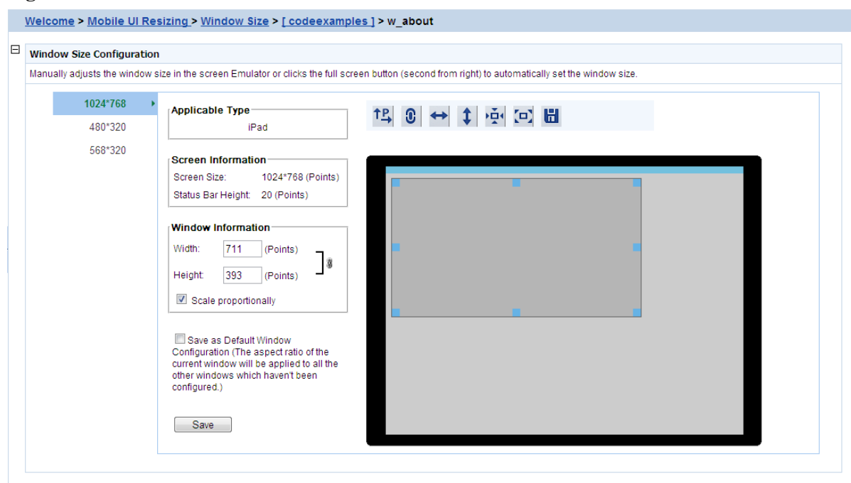
Figure 5.119: Screen emulator
