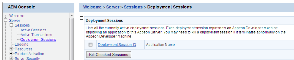
Figure 5.10: Deployment Sessions
