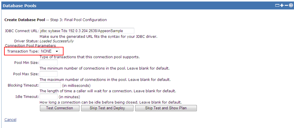
Figure 4.46: Final
