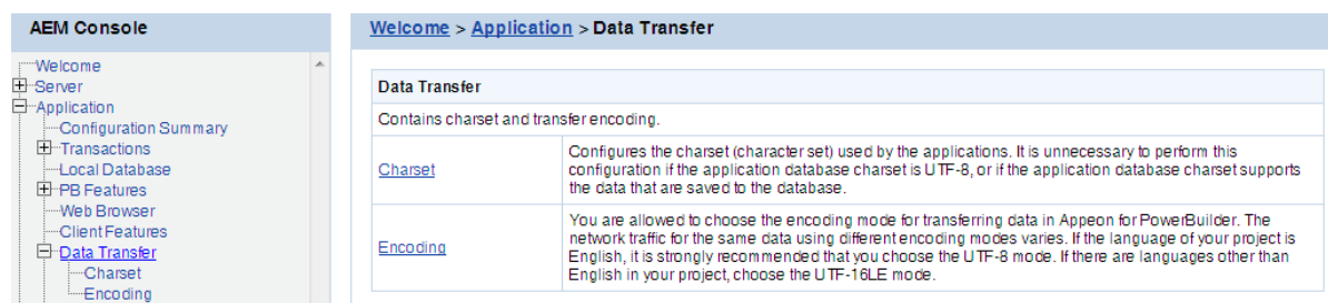
Figure 5.91: Data Transfer
