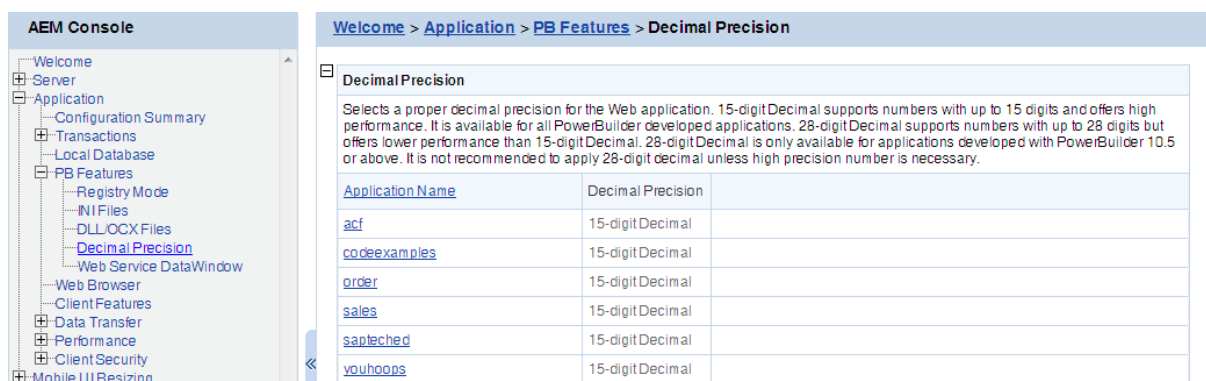
Figure 5.72: Decimal Precision
