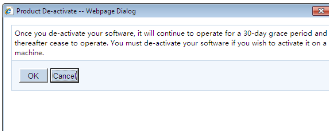
Figure 5.27: Product De-activate
