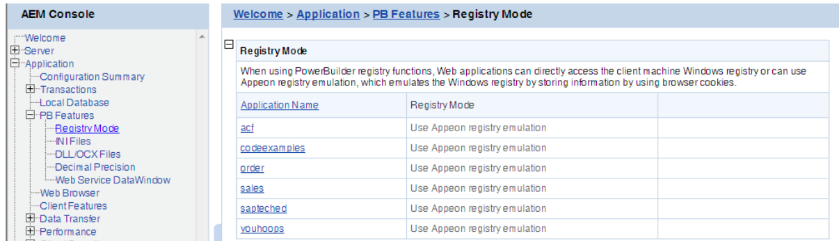
Figure 5.64: Registry Mode
