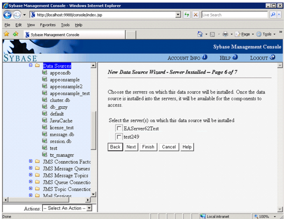
Figure 4.79: Server installed
