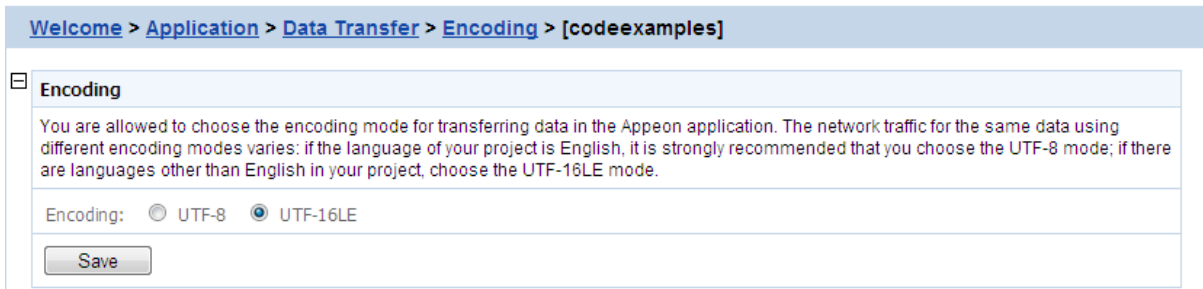
Figure 5.96: Encoding settings
