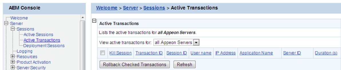
Figure 5.9: Active Transactions
