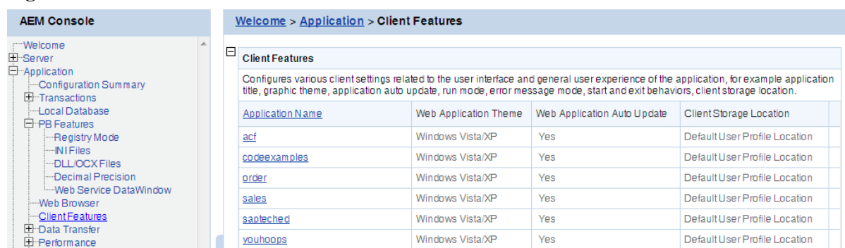
Figure 5.80: Client Features
