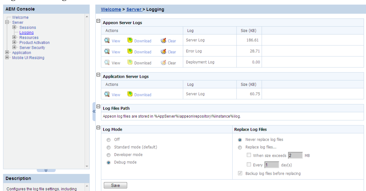
Figure 5.11: Logs
