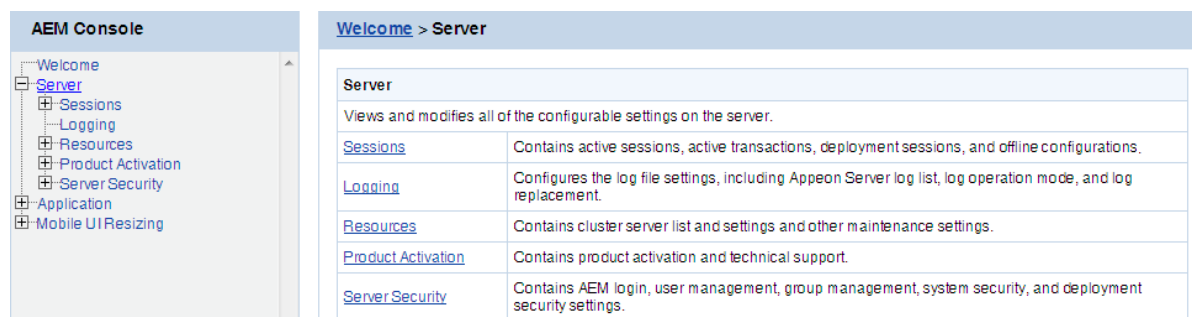
Figure 5.6: Server
