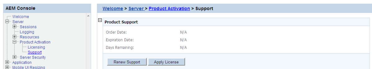
Figure 5.33: Support
