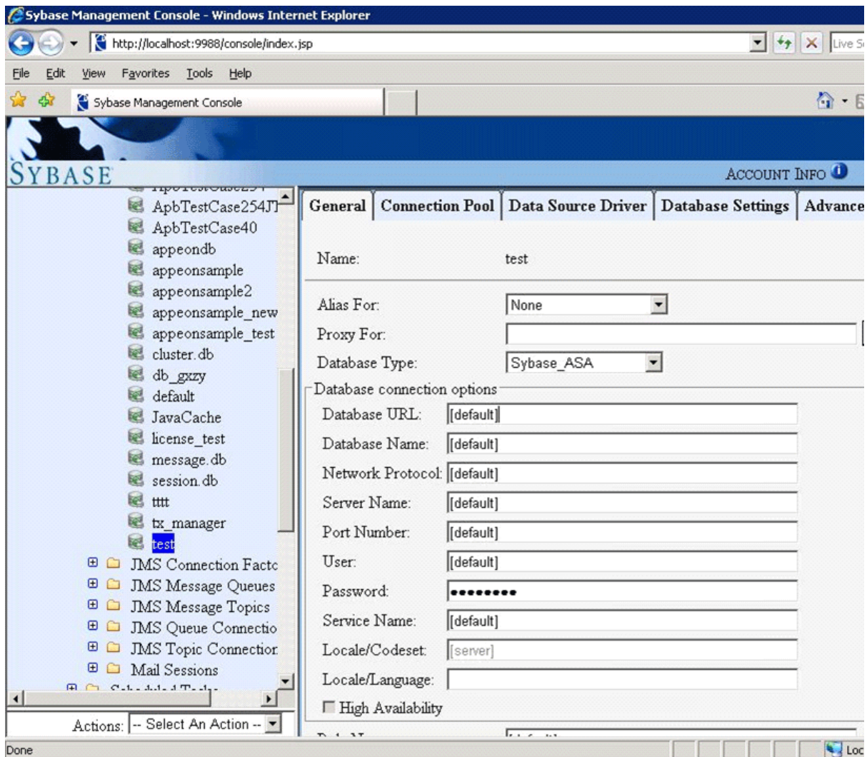
Figure 4.81: Database URL
