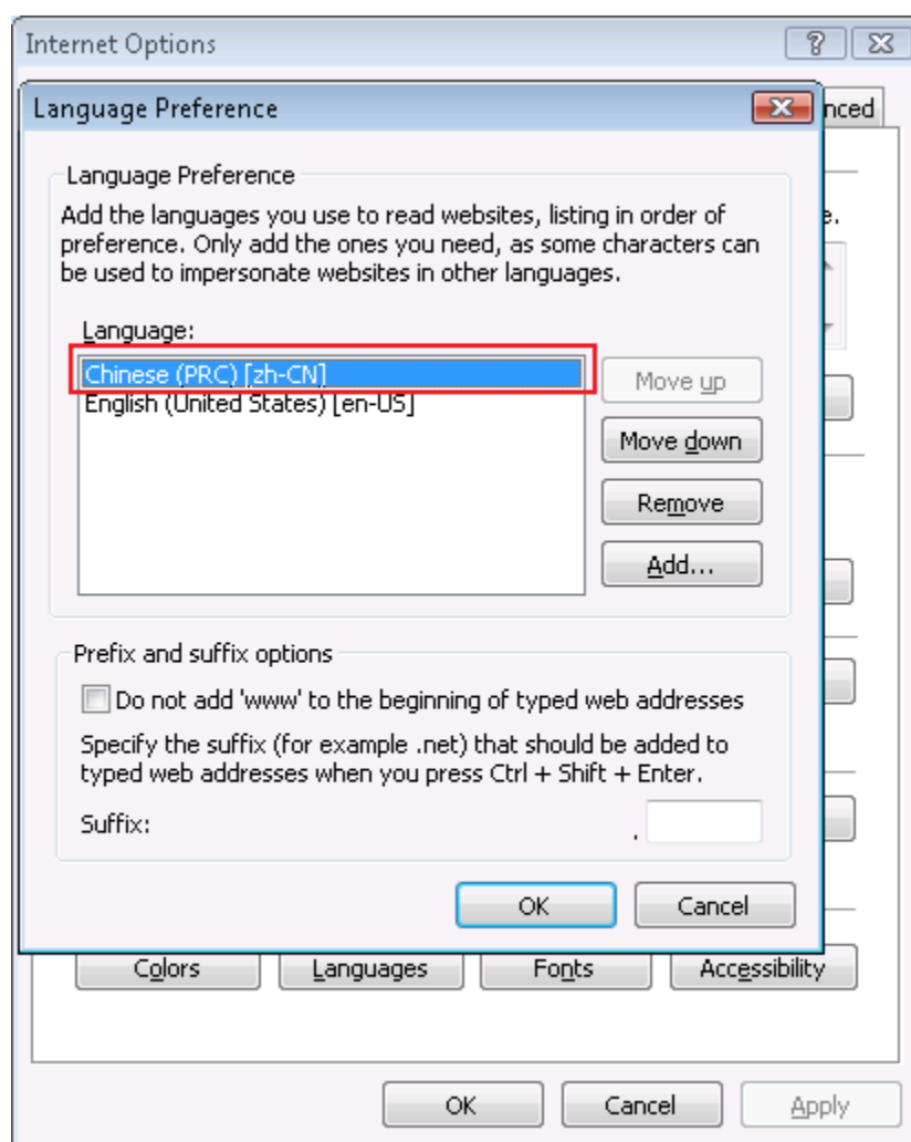
Figure 5.3: Language settings
