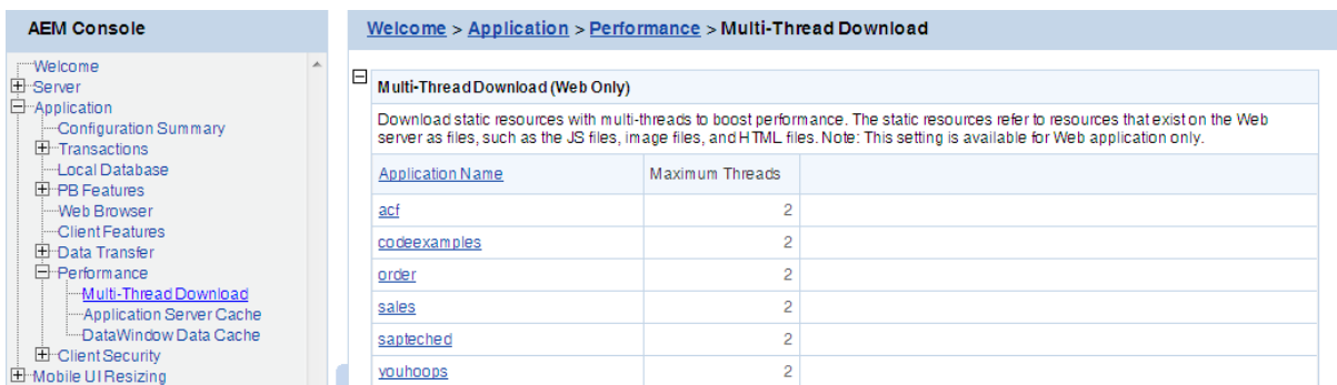
Figure 5.98: Multi-thread Download
