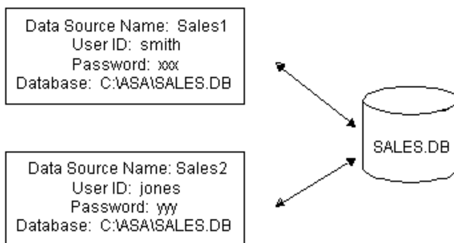
Figure: Using two data sources to access a database
