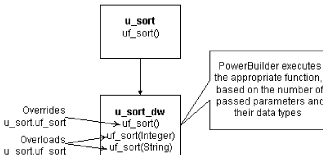
Figure: Function overloading
