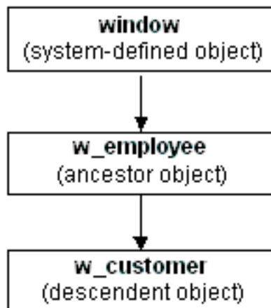
Figure: Window inheritance hierarchy
