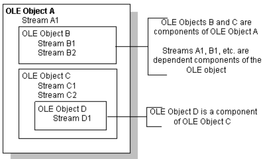
Figure: OLE storage structure
