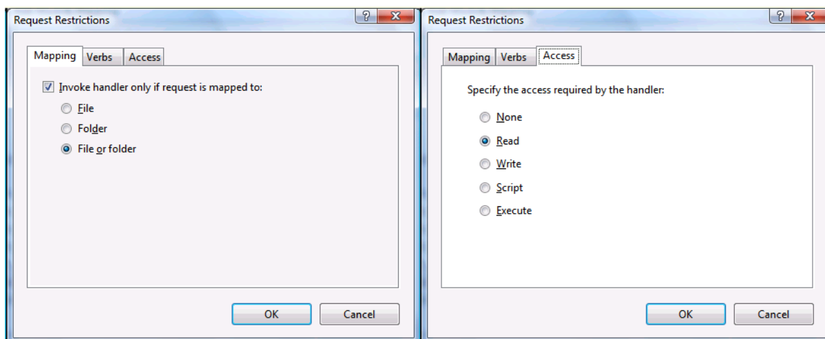
Figure 4.8: Request restrictions
