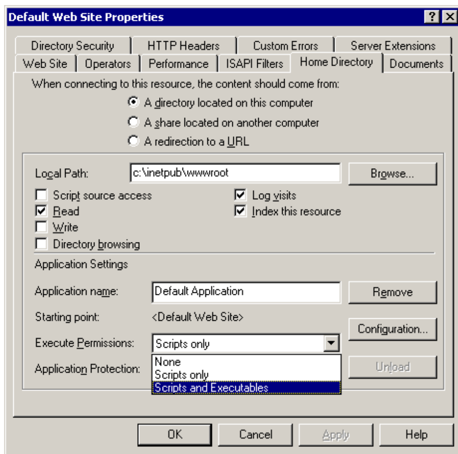
Figure 4.18: Home Directory
