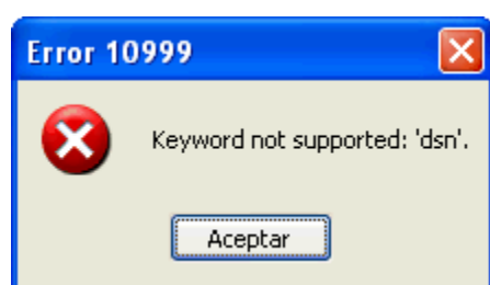
Figure 4.19: Error 10999
