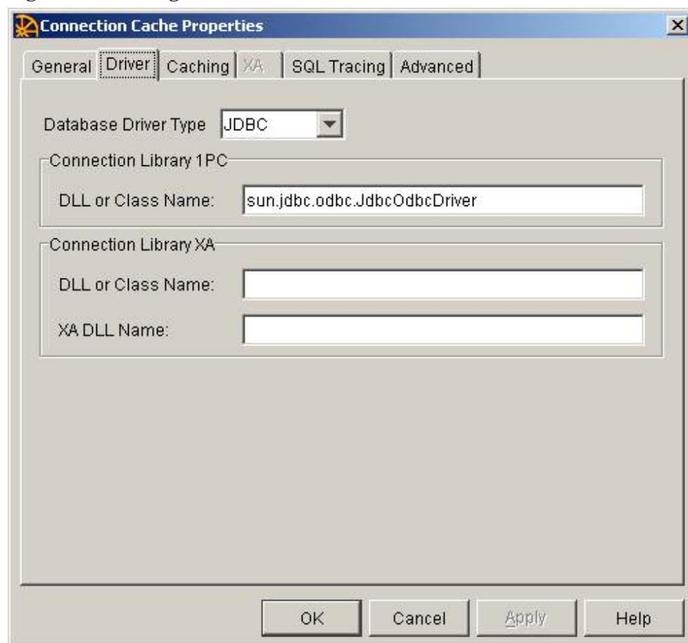
Figure 5.29: Configure Driver
