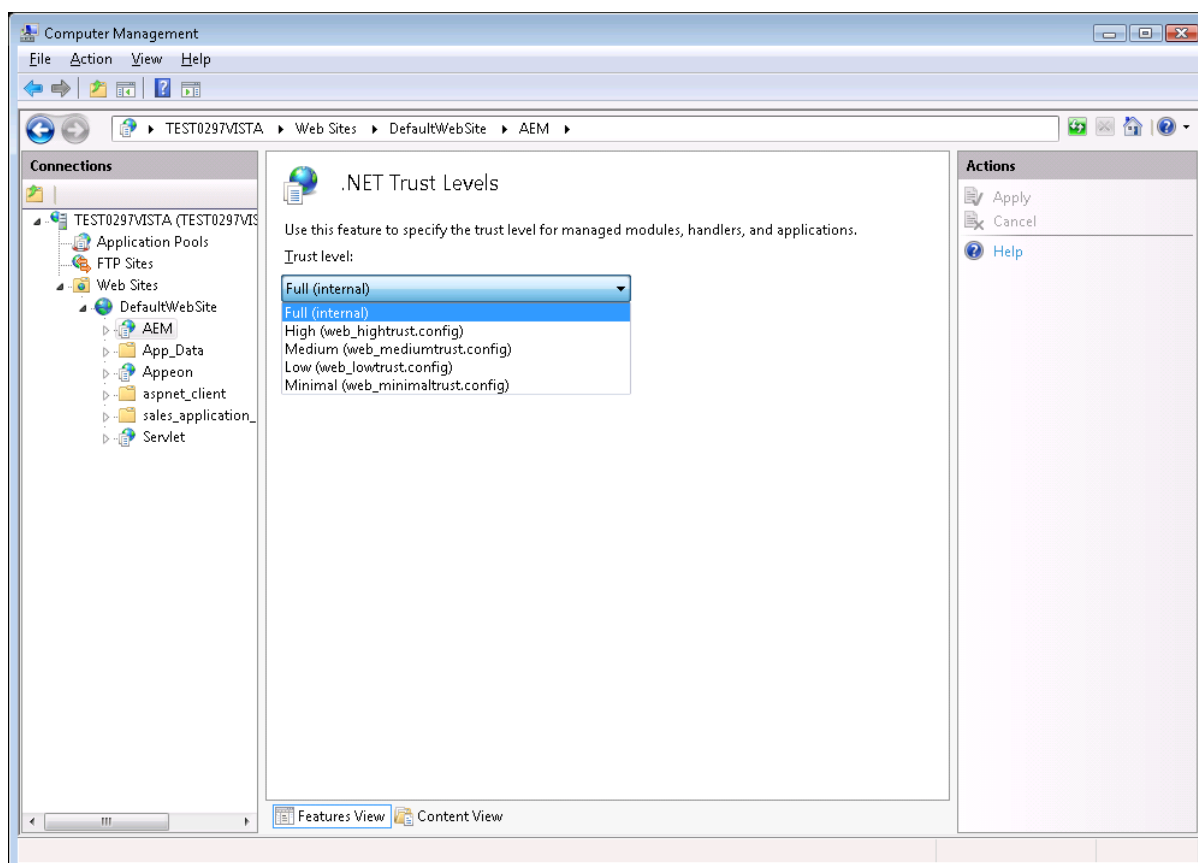
Figure 1.2: Full (internal)
