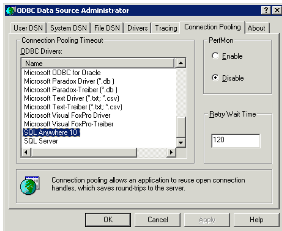
Figure 4.26: Connection Pooling
