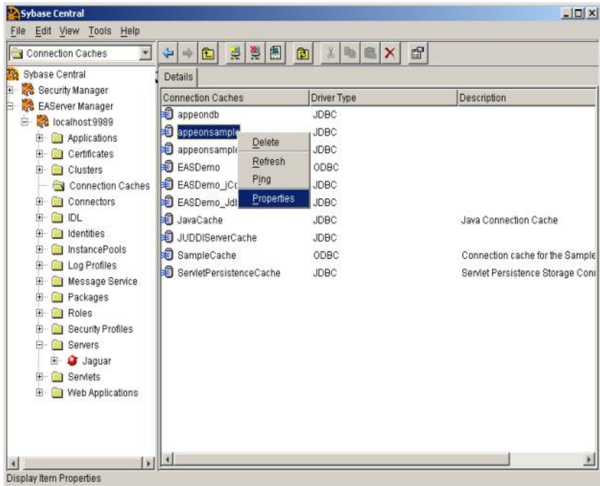
Figure 5.27: Select Properties
