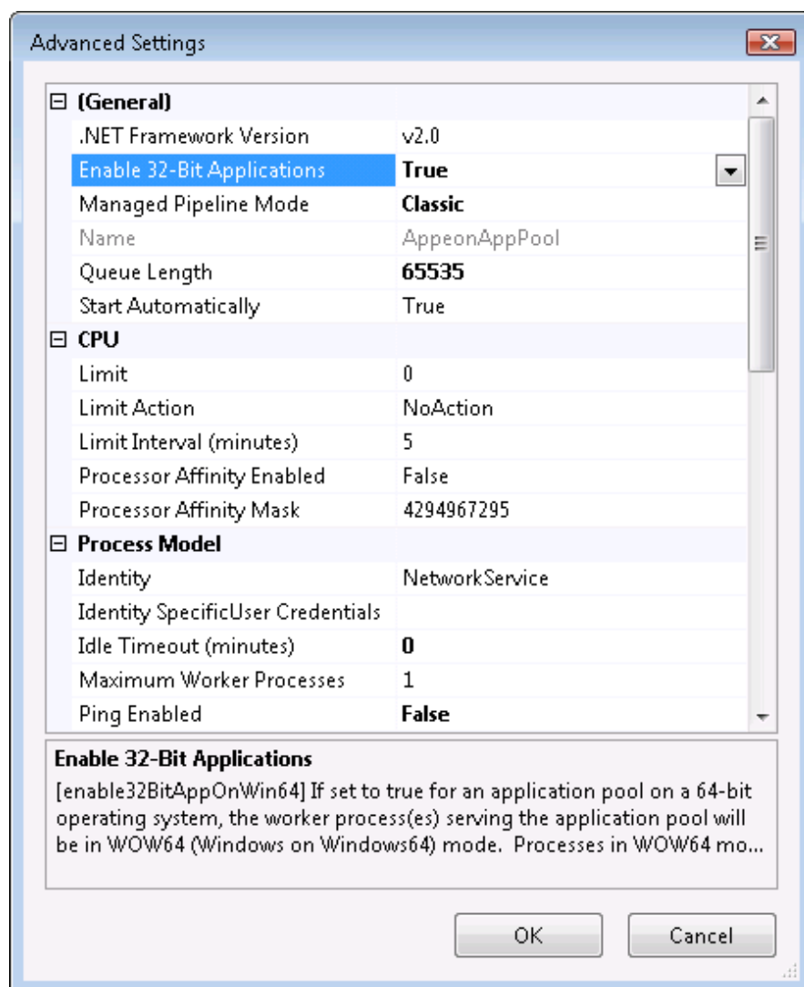
Figure 1.13: Advanced settings
