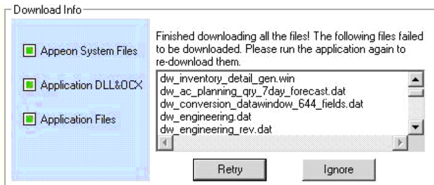
Figure 4.4: Download info
