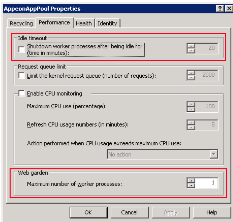
Figure 1.7: Performance
