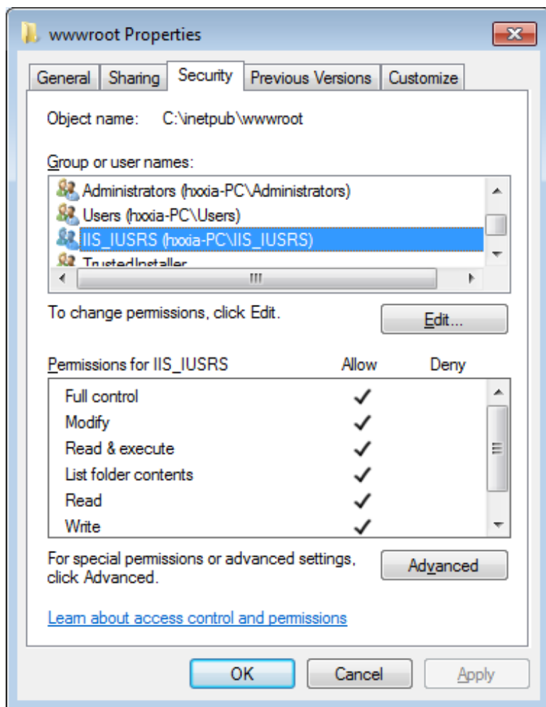
Figure 1.10: Security
