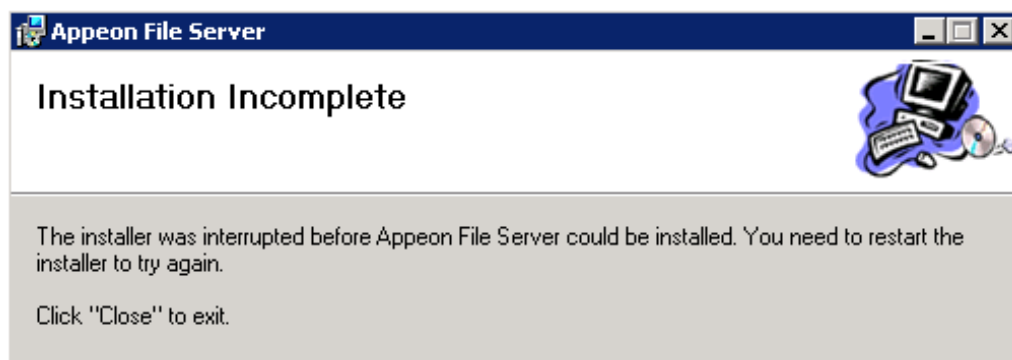
Figure 1.15: Installation incomplete
