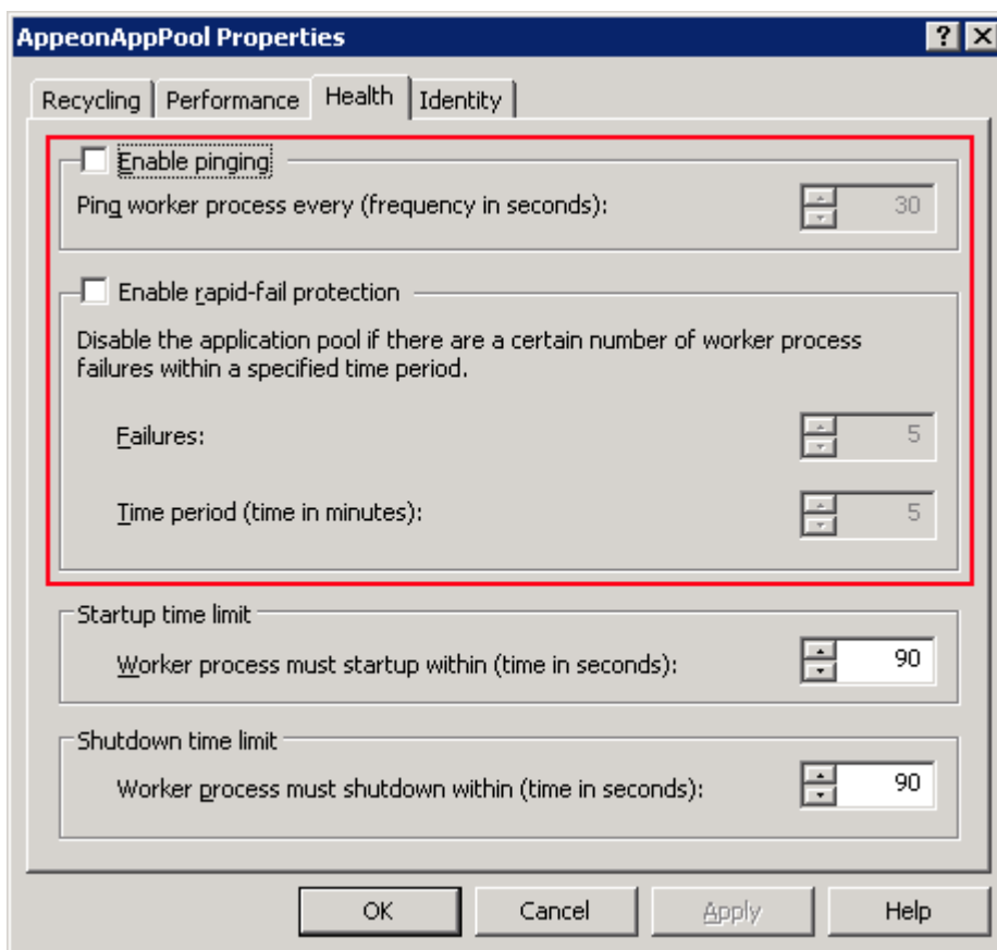
Figure 1.8: Health
