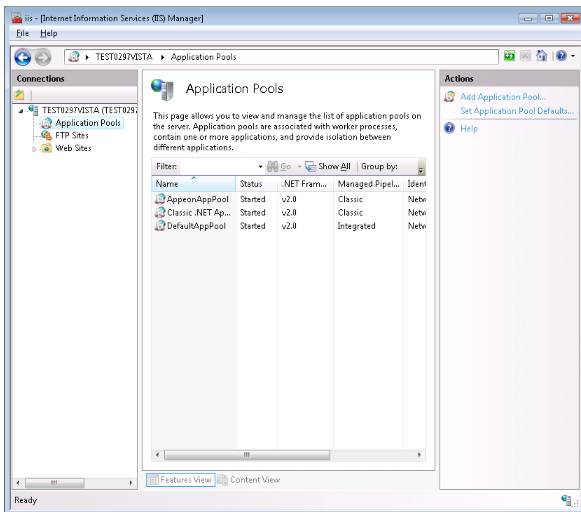
Figure 1.12: Application pools
