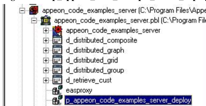
Figure 4.17: p_appeon_code_example_server_deploy
