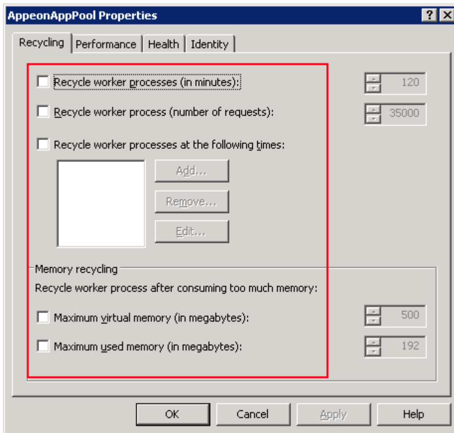
Figure 1.6: Recycling
