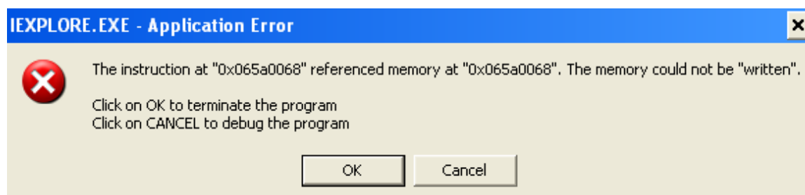
Figure 4.10: IE 8 crashes
