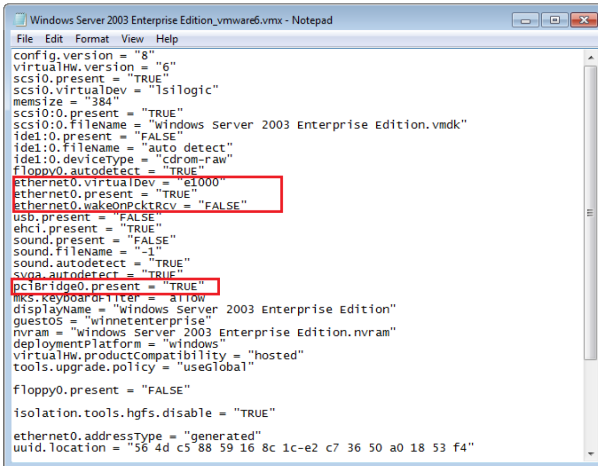
Figure 5.22: Copy address
