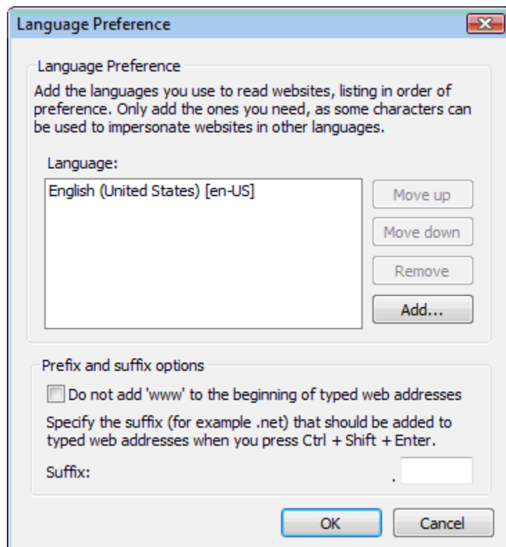
Figure 5.10: Language Preference
