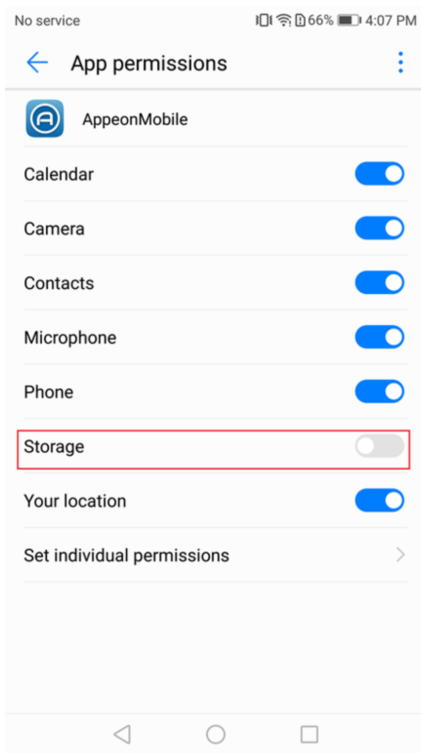
Figure 4.1: Storage permission
