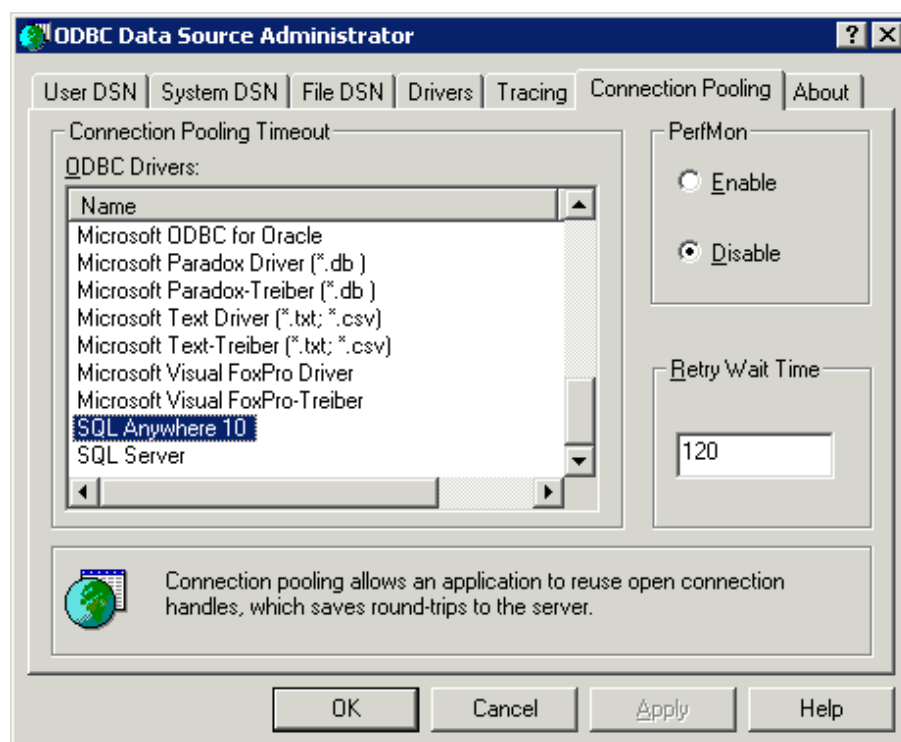
Figure 4.24: Connection Pooling
