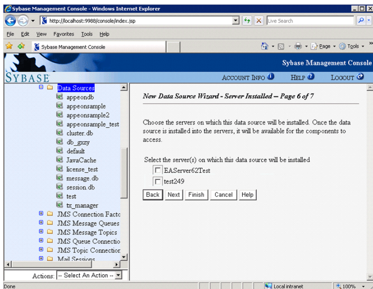
Figure 4.73: Server installed
