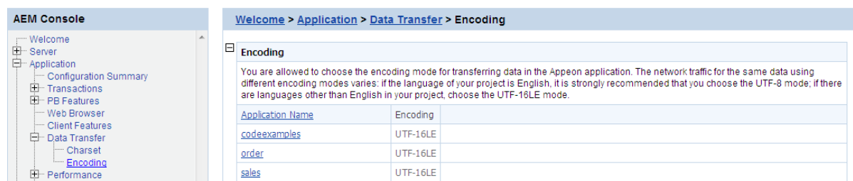
Figure 5.93: Encoding
