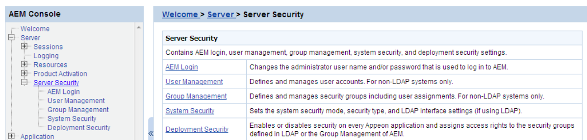
Figure 5.38: Server Security
