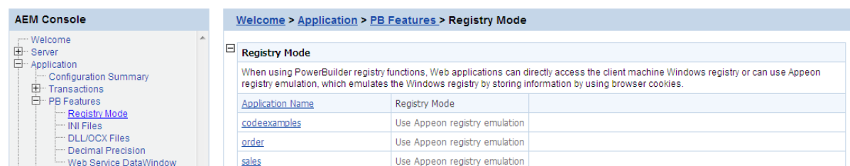
Figure 5.62: Registry Mode
