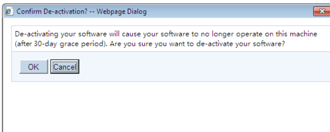
Figure 5.27: Confirm De-activation
