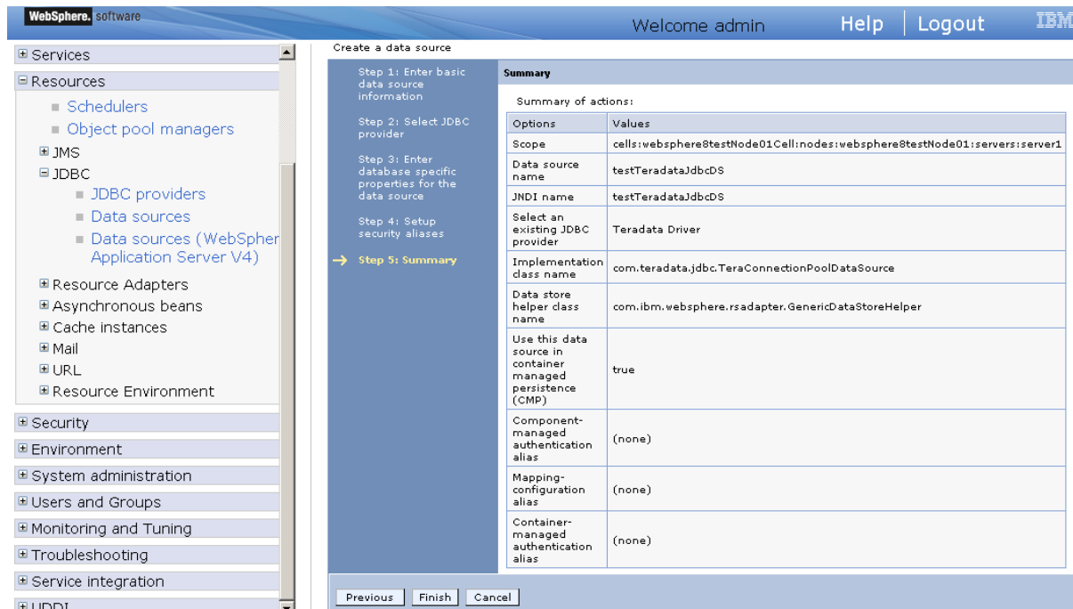
Figure 4.37: Summary page
