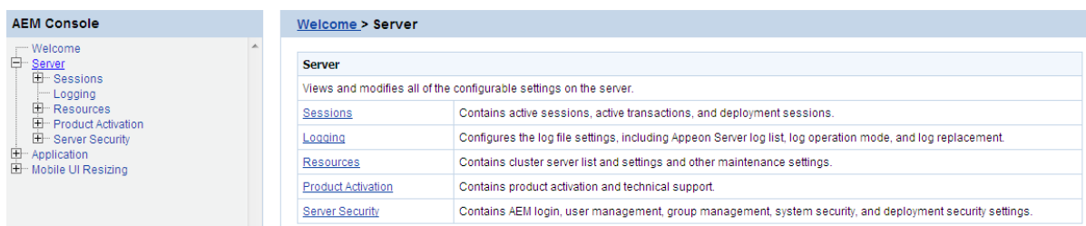
Figure 5.5: Server
