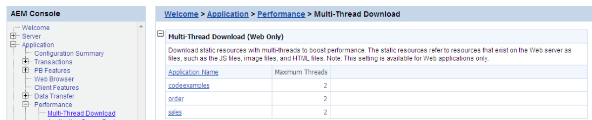
Figure 5.96: Multi-thread Download
