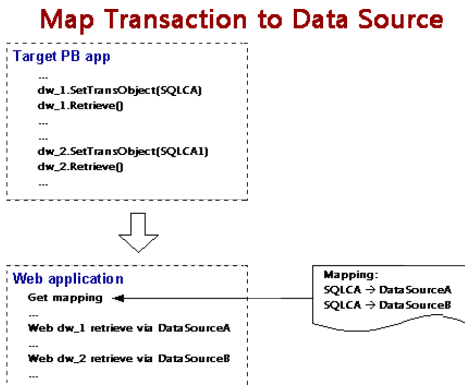
Figure 4.76: Map transaction to data source
