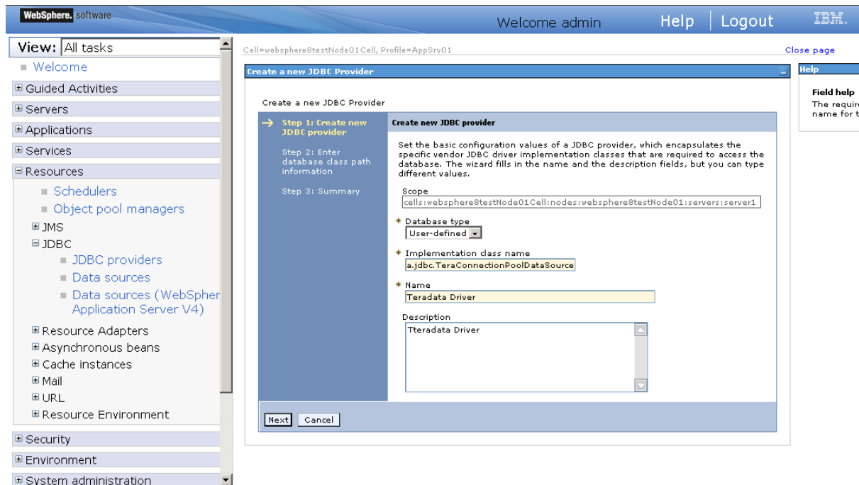
Figure 4.27: Create new JDBC provider page
