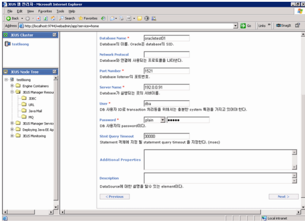
Figure 4.66: Datasource properties page
