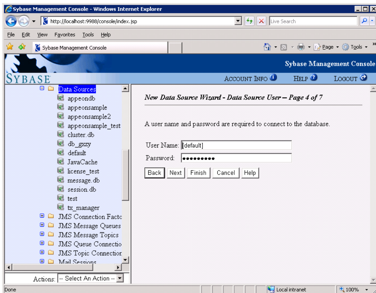
Figure 4.71: Database user name and password
