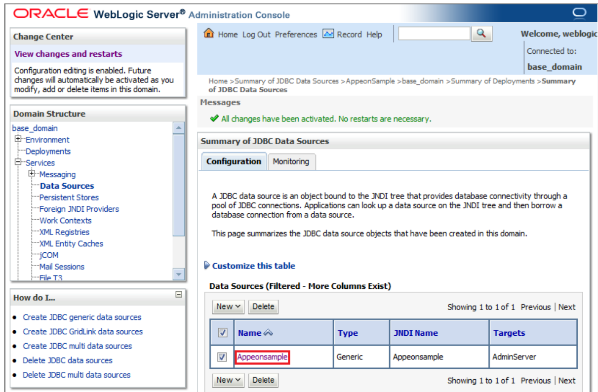
Figure 4.16: Summary of JDBC Data Sources page
