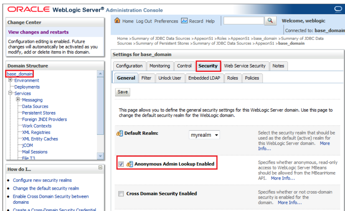
Figure 4.17: Settings for the base_domain page
