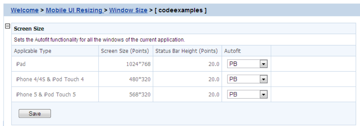
Figure 5.112: Screen size list
