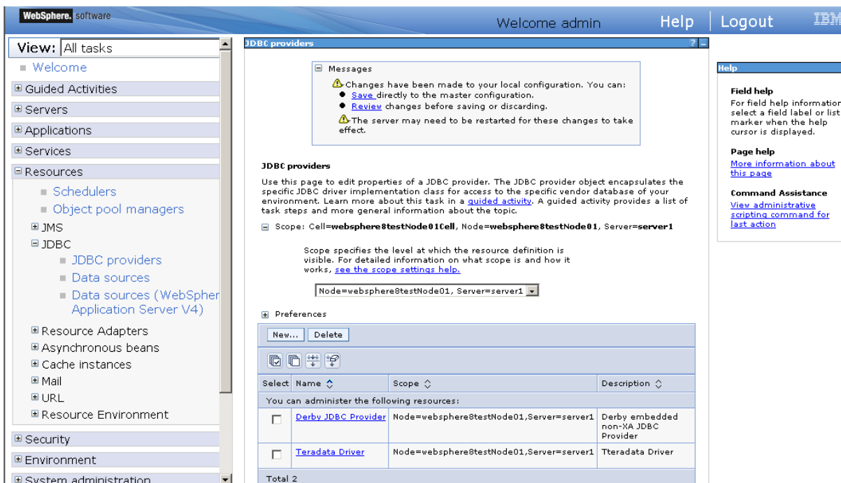
Figure 4.30: JDBC providers page
