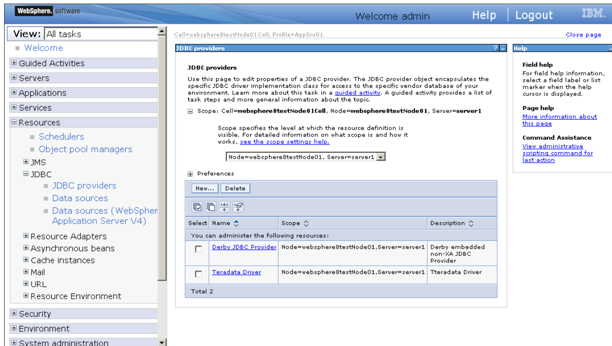
Figure 4.31: The newly created JDBC providers page
