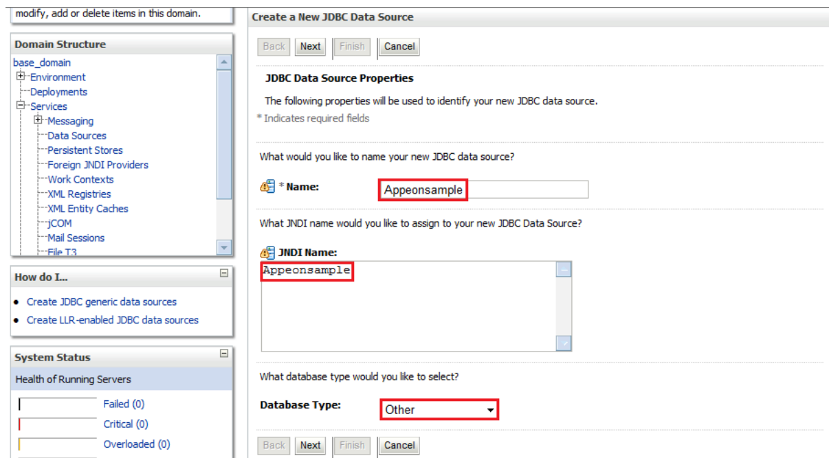
Figure 4.10: JDBC Data Source Properties page
