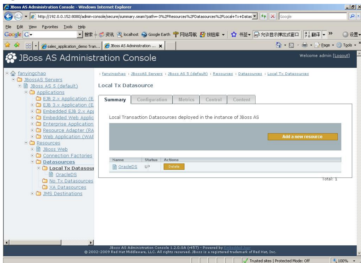
Figure 4.56: Add a new datasource
