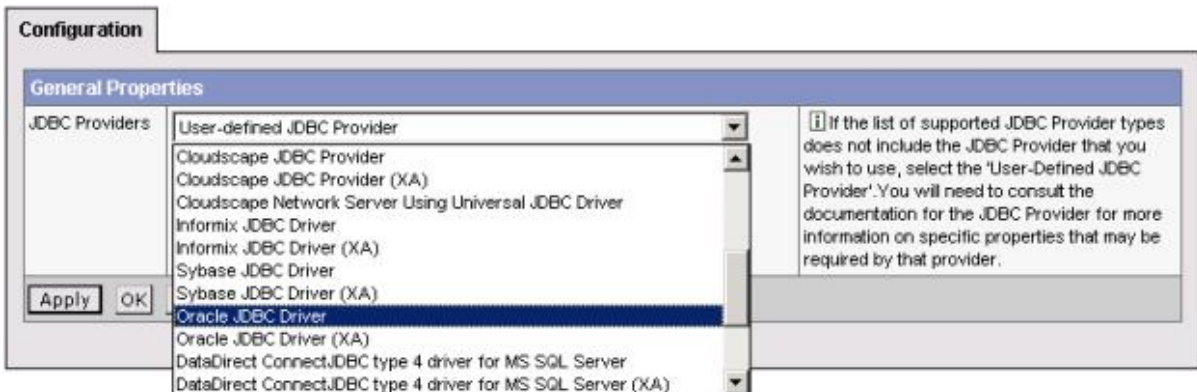
Figure 4.20: Select JDBC Provider type
