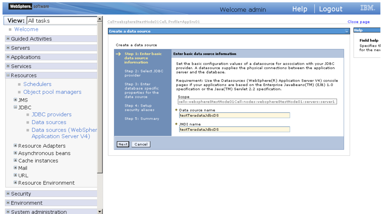
Figure 4.33: Enter basic data source information page
