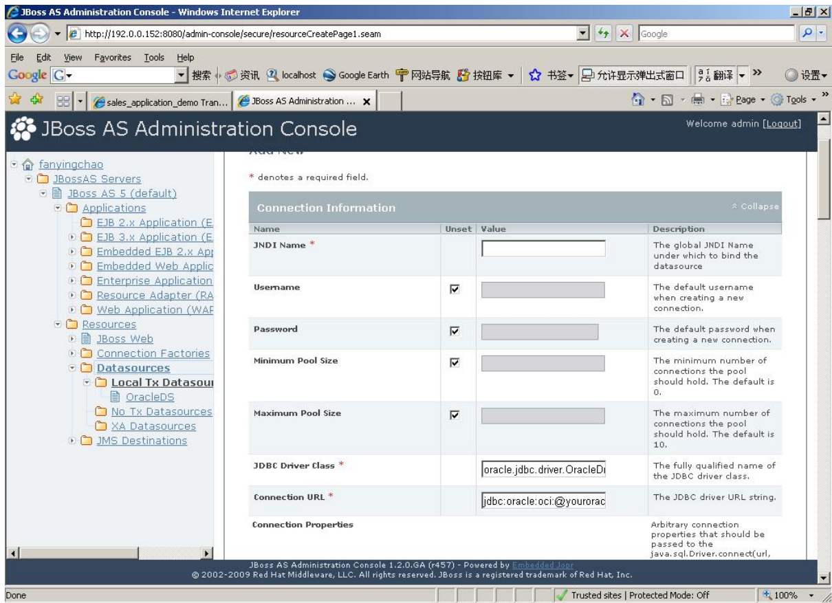
Figure 4.58: Specify connection information
