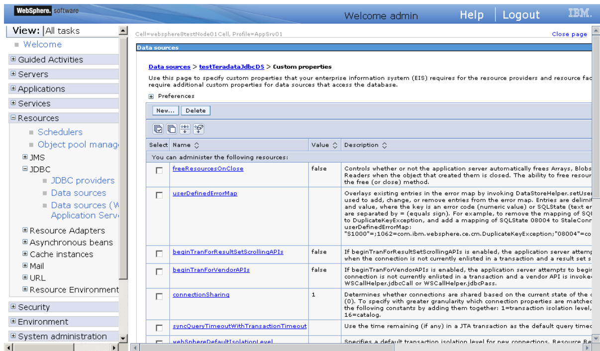
Figure 4.41: Custom properties page
