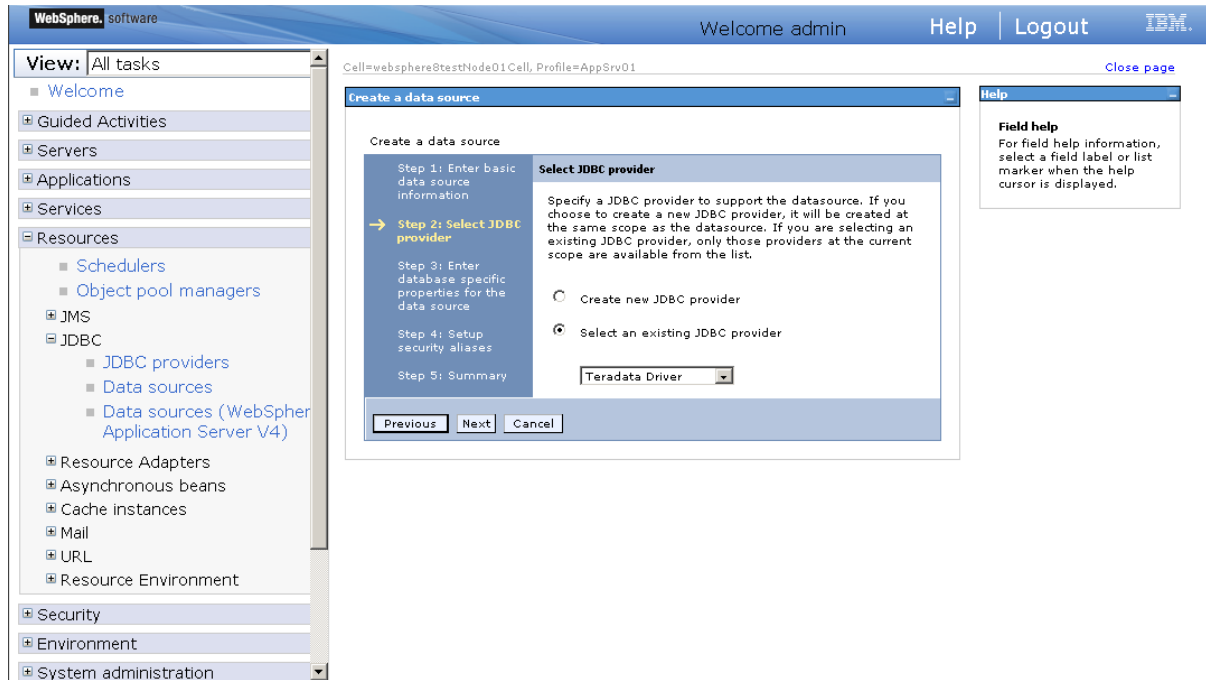
Figure 4.34: Select JDBC provider page
