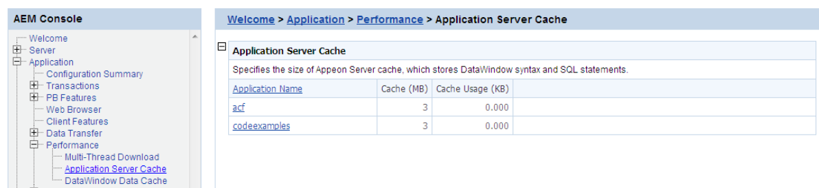
Figure 5.98: Application Server Cache
