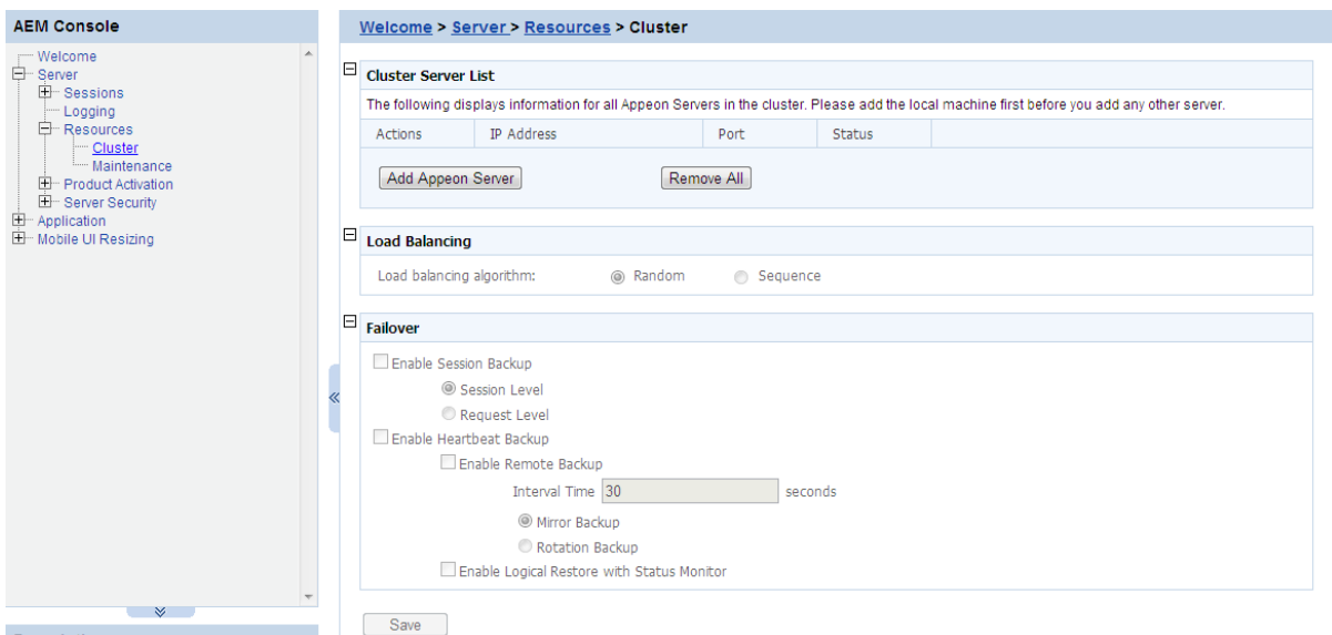
Figure 5.13: Cluster
