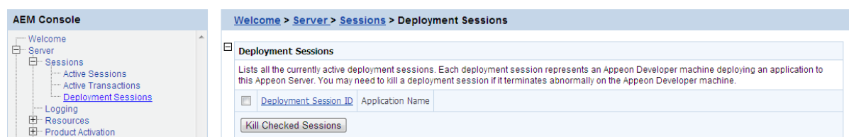
Figure 5.9: Deployment Sessions
