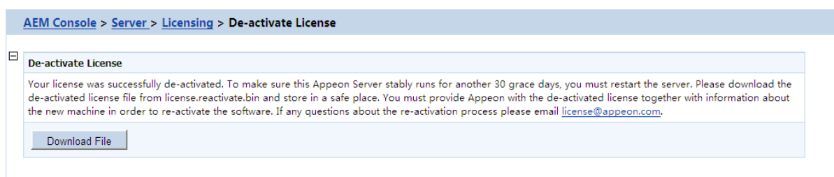
Figure 5.28: De-activate License
