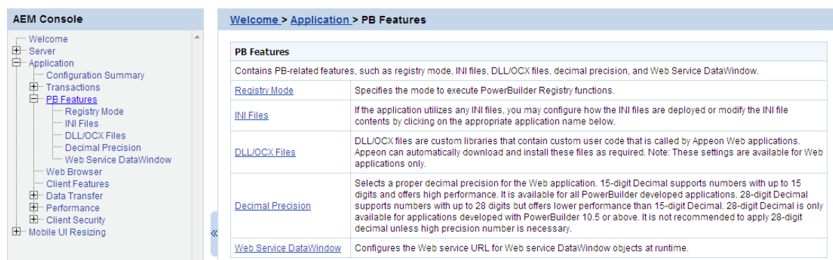
Figure 5.61: PB Features
