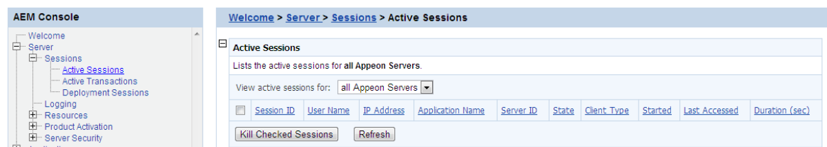
Figure 5.7: Active Sessions
