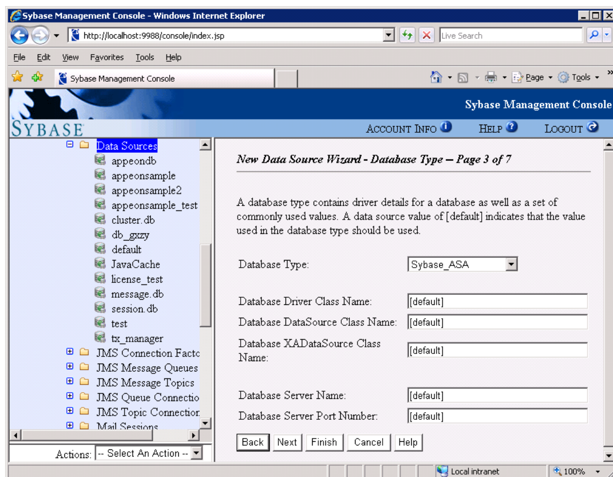
Figure 4.70: Database type
