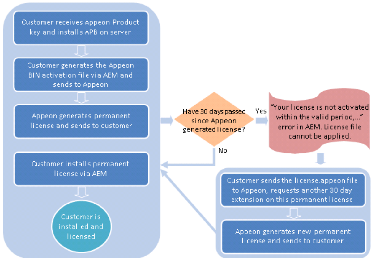
Figure 5.19: Activation process
