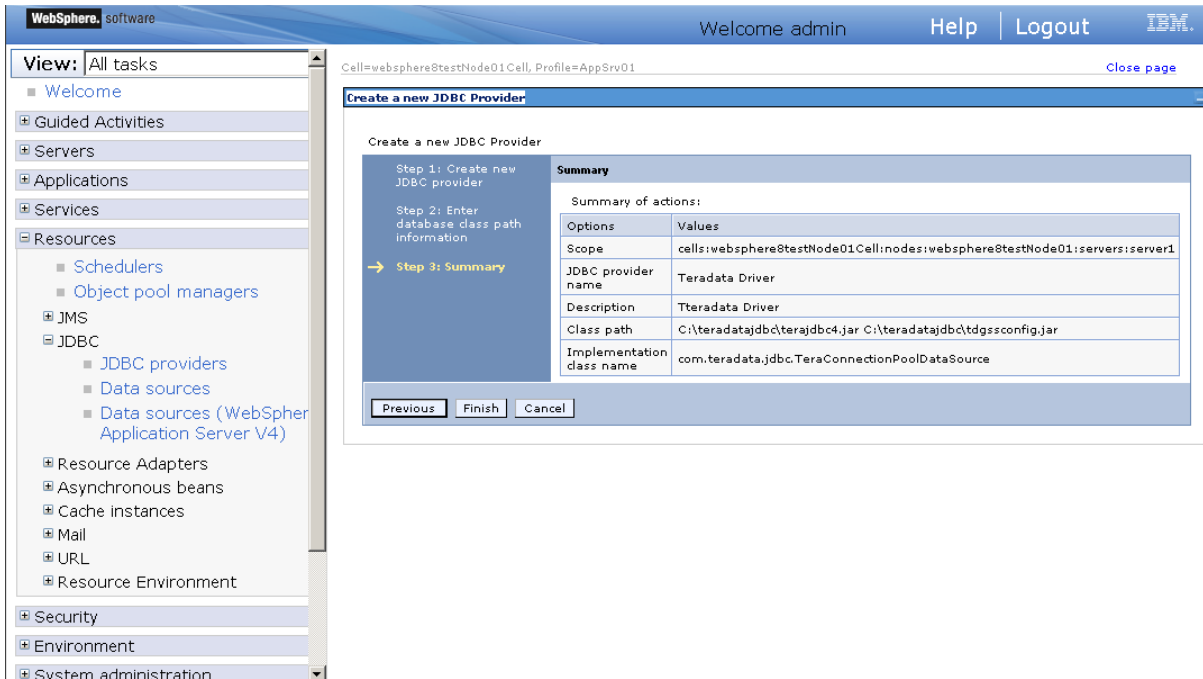
Figure 4.29: Summary page
