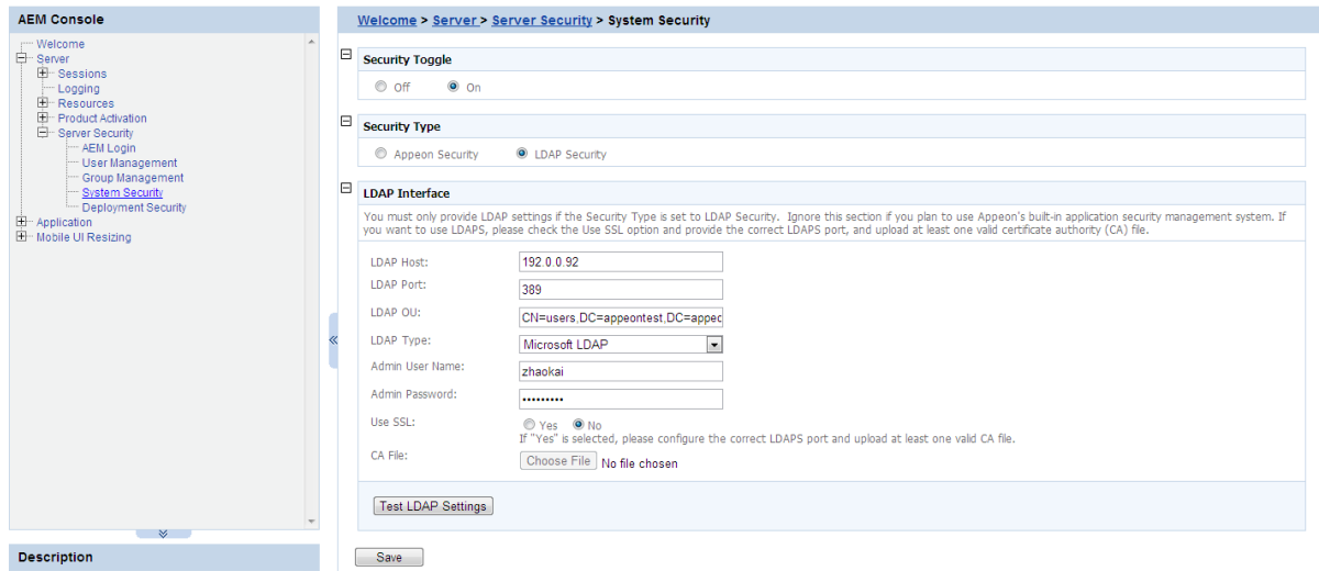
Figure 5.50: System Security
