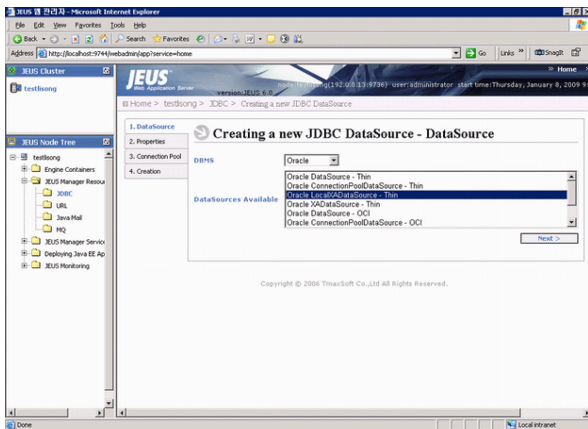
Figure 4.65: Creating a new JDBC DataSource page
