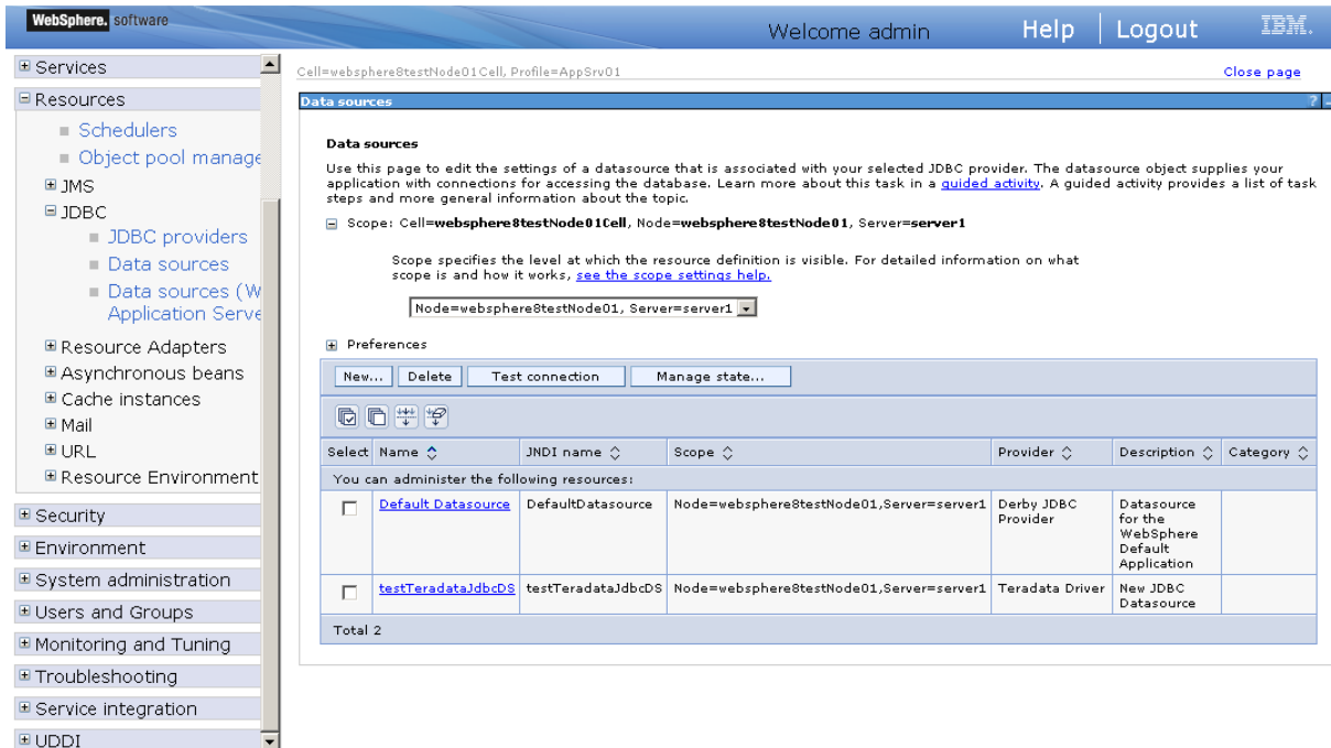
Figure 4.39: The newly created data source information page
