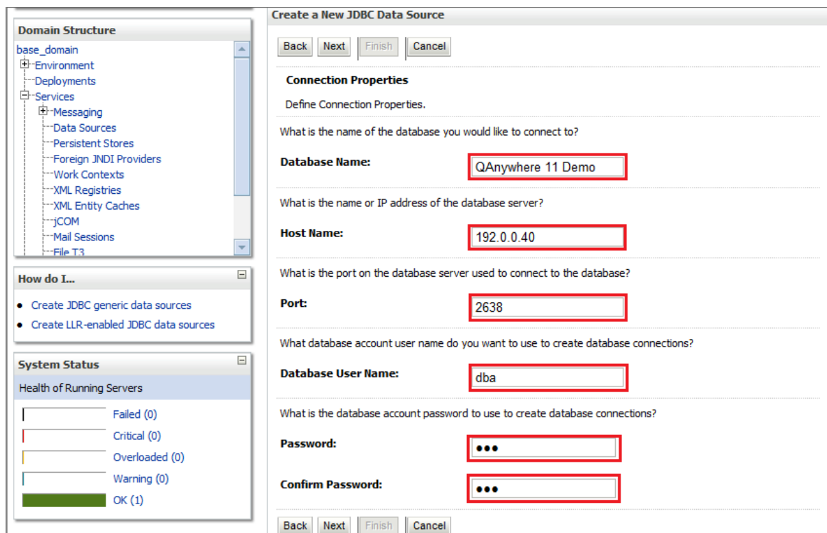
Figure 4.13: Connection Properties page
