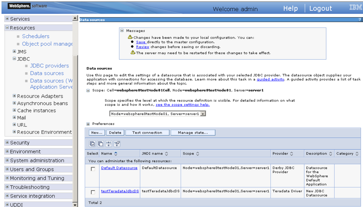
Figure 4.38: Data Sources page
