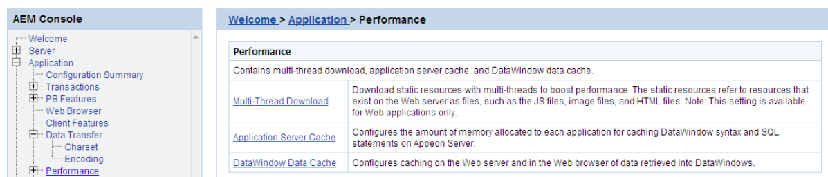
Figure 5.95: Performance
