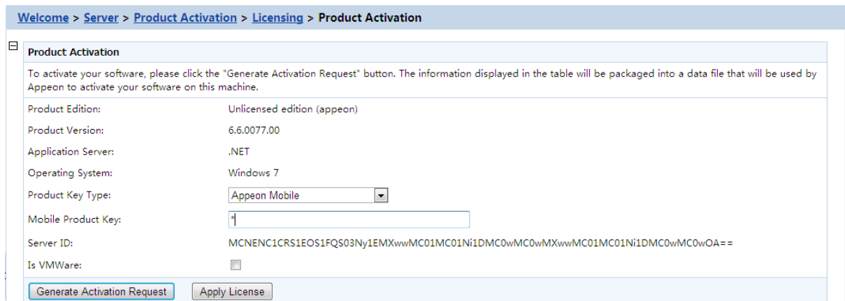
Figure 5.20: Product activation
