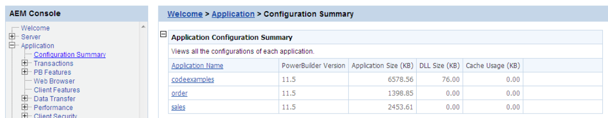
Figure 5.53: Application Summary
