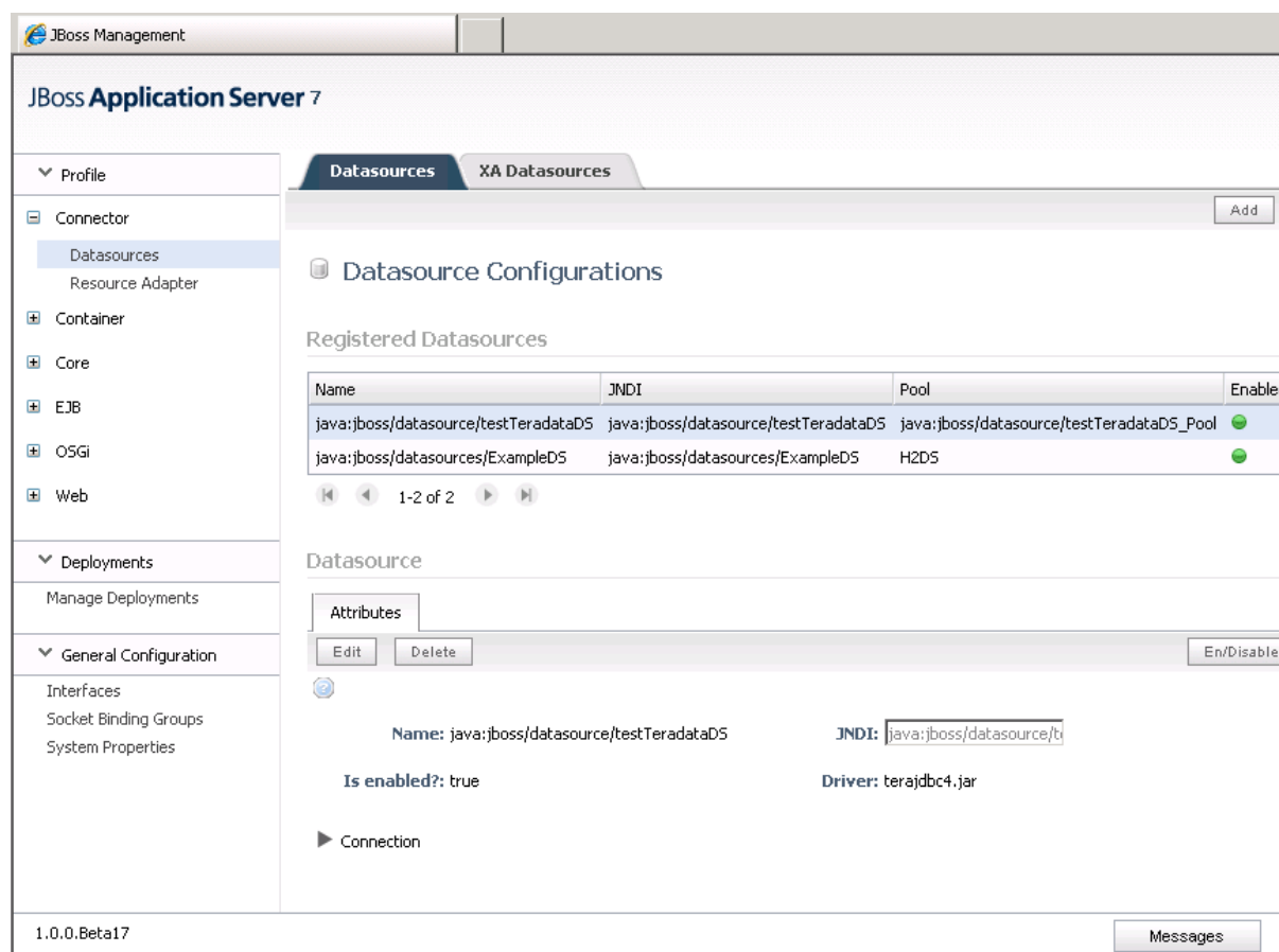
Figure 4.55: Datasource list
