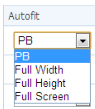
Figure 5.113: Autofit mode
