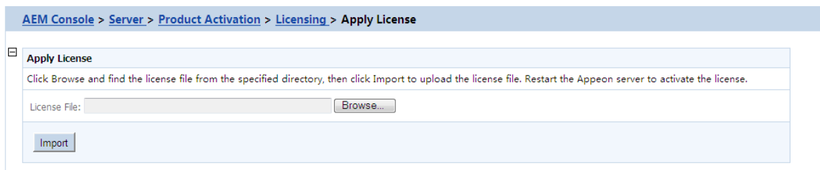
Figure 5.32: Apply license
