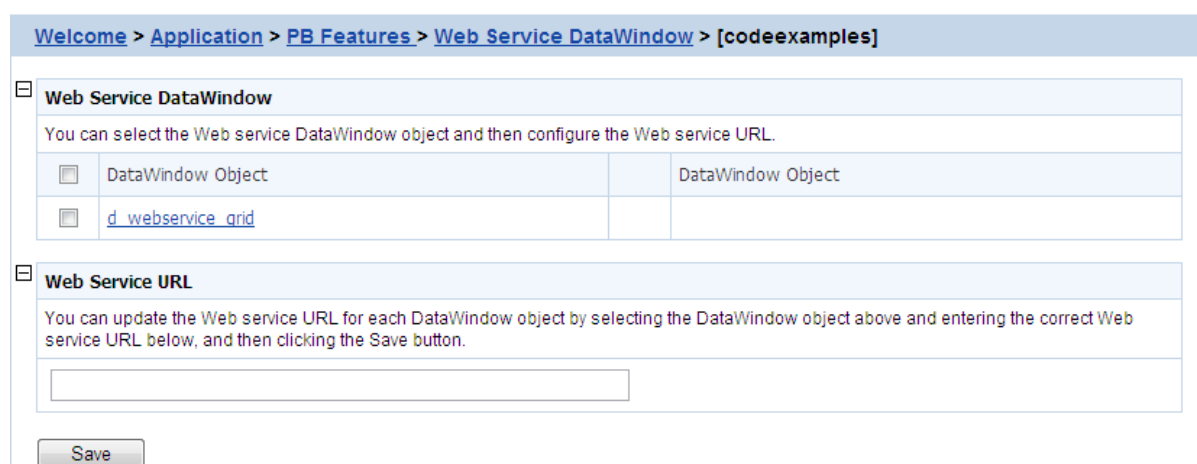
Figure 5.73: Web service DataWindow for apeon_code_examples
