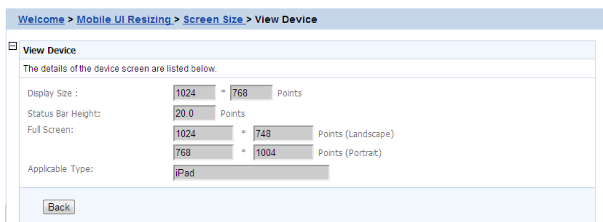
Figure 5.110: Screen details
