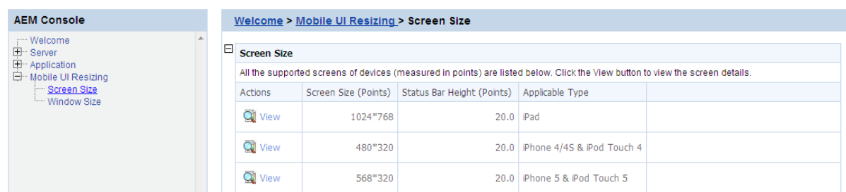
Figure 5.109: Screen Size
