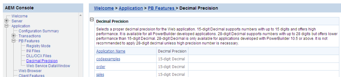
Figure 5.70: Decimal Precision
