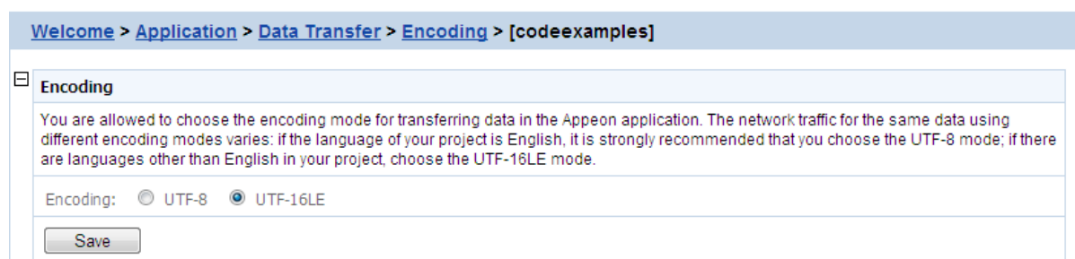
Figure 5.94: Encoding settings
