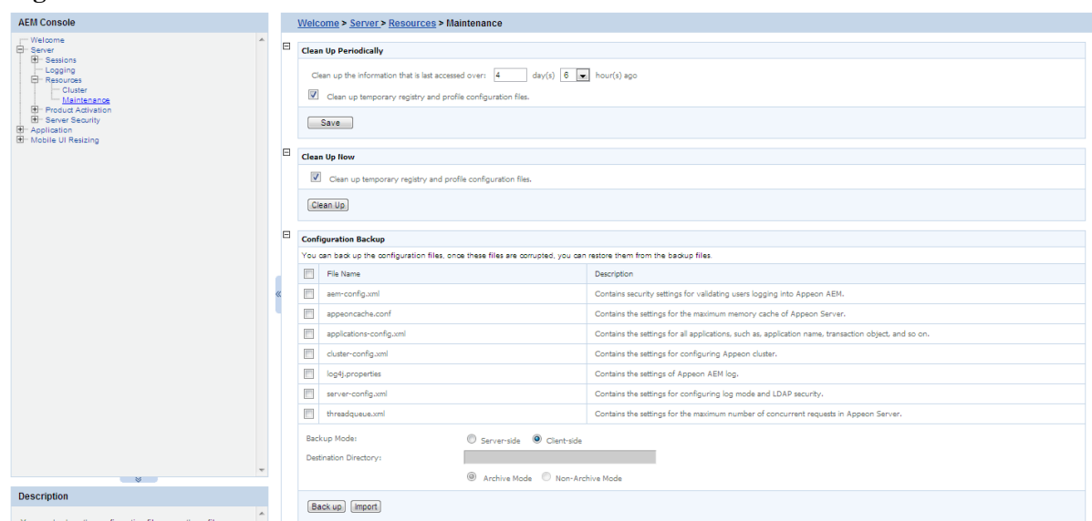
Figure 5.15: Maintenance
