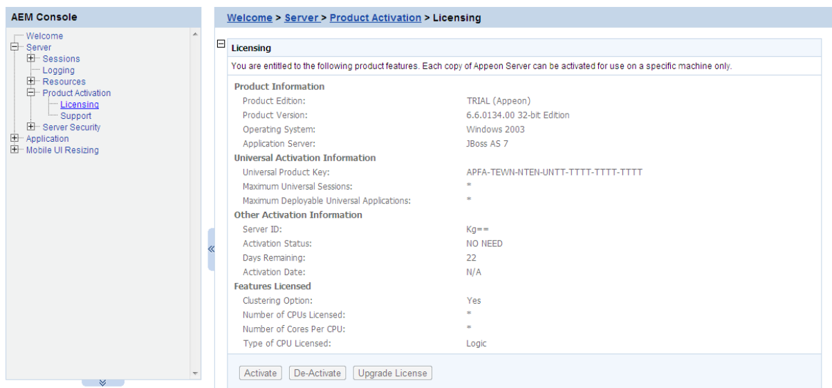
Figure 5.18: Licensing
