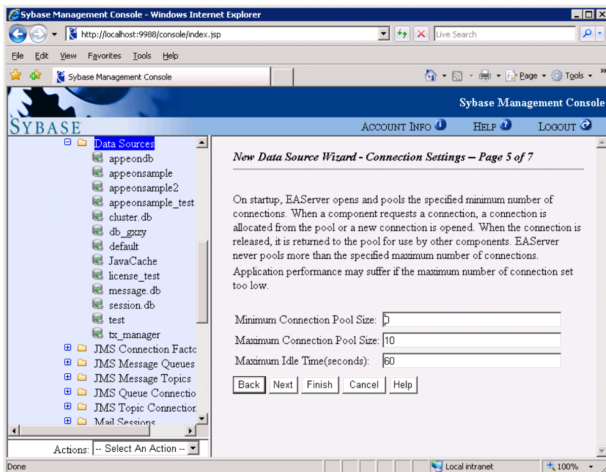
Figure 4.72: Connection settings
