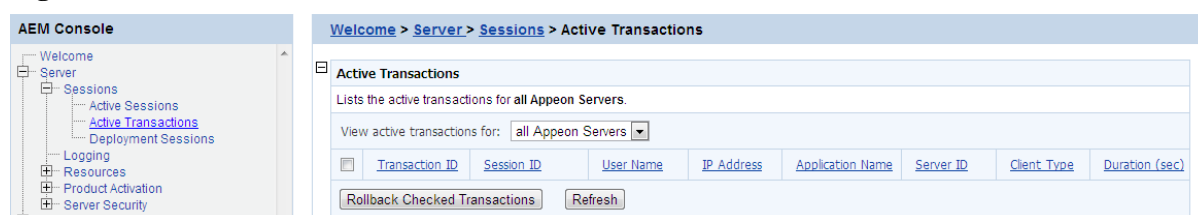
Figure 5.8: Active Transactions
