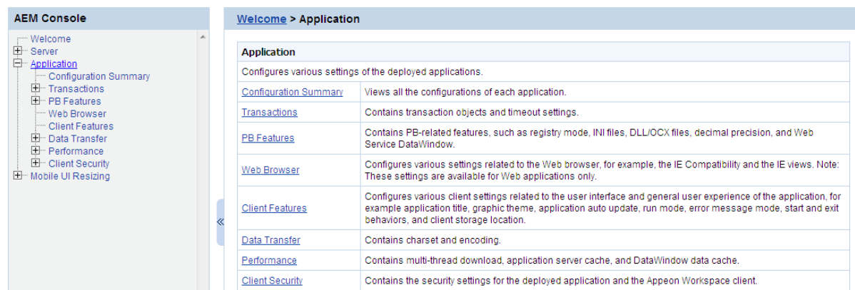
Figure 5.52: Application
