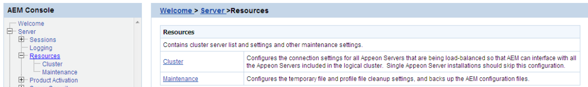
Figure 5.12: Resource
