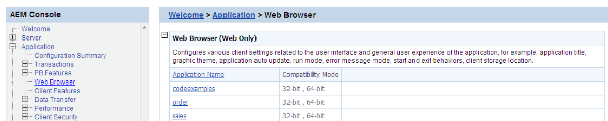
Figure 5.75: Web Browser
