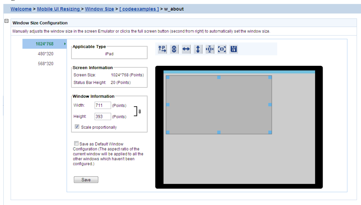
Figure 5.115: Screen emulator
