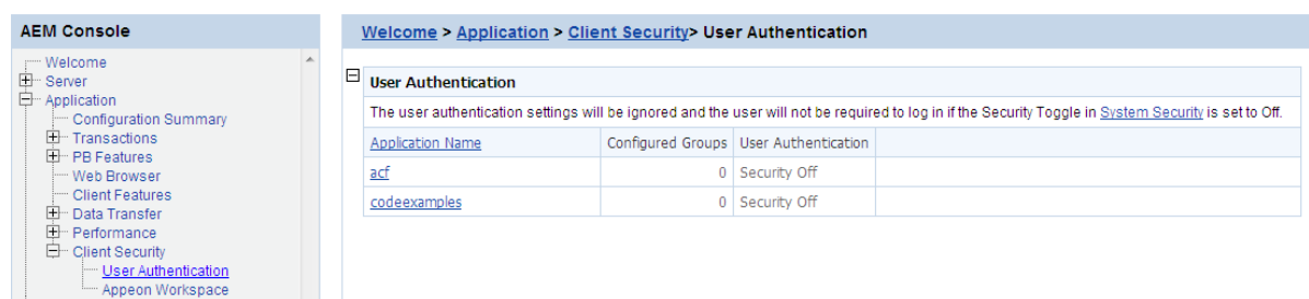
Figure 5.104: Application Security
