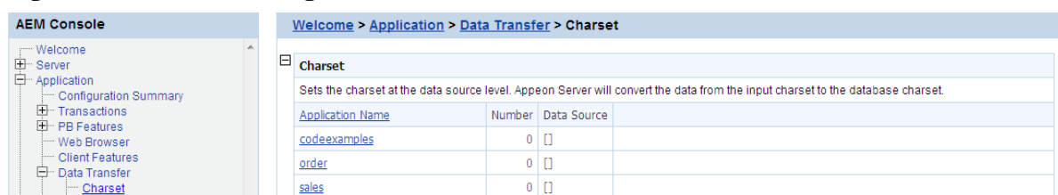
Figure 5.90: Charset settings
