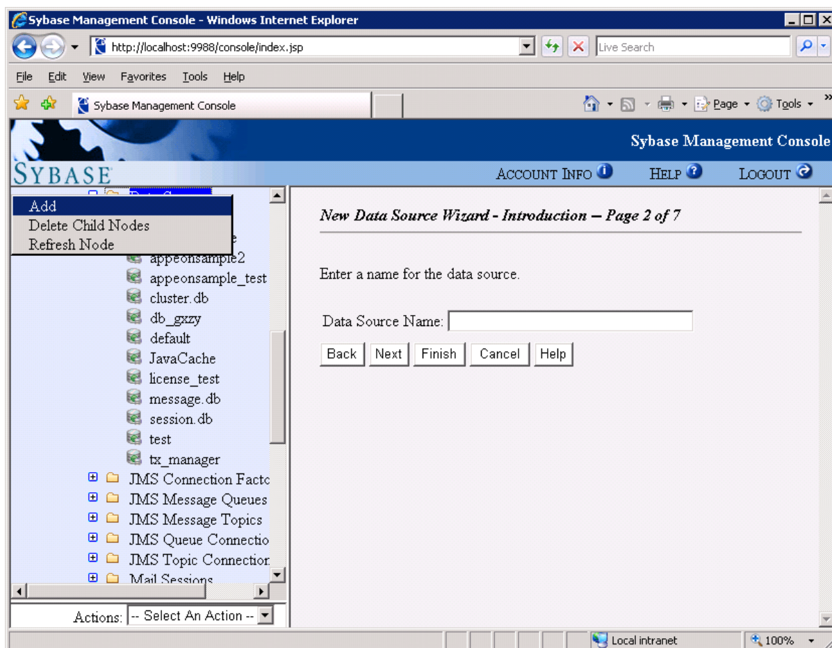
Figure 4.69: Datasource name
