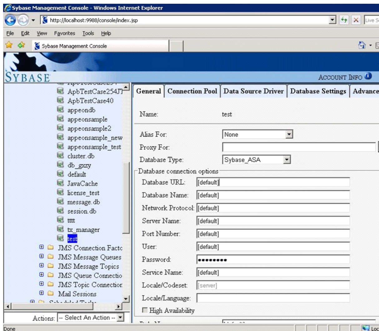
Figure 4.75: Database URL
