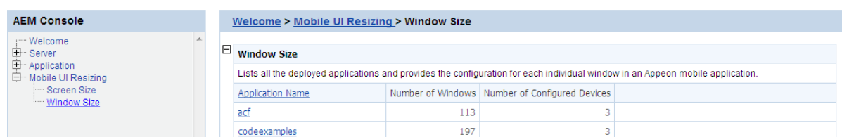
Figure 5.111: Window size
