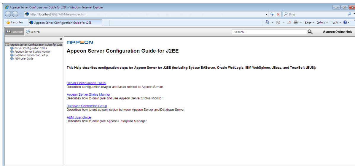
Figure 5.4: Appeon Help
