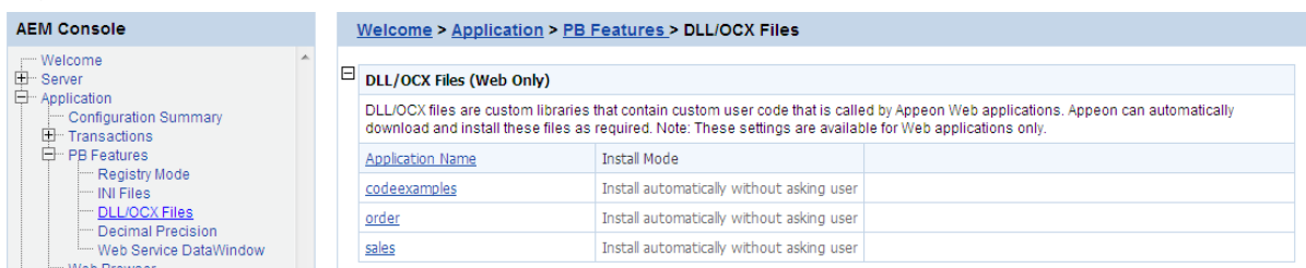
Figure 5.68: DLL/OCX Files
