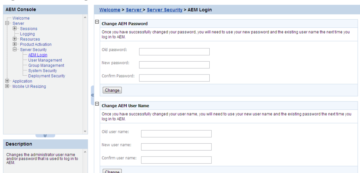
Figure 5.39: AEM Login
