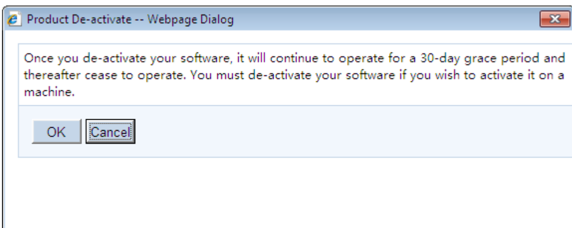
Figure 5.26: Product De-activate
