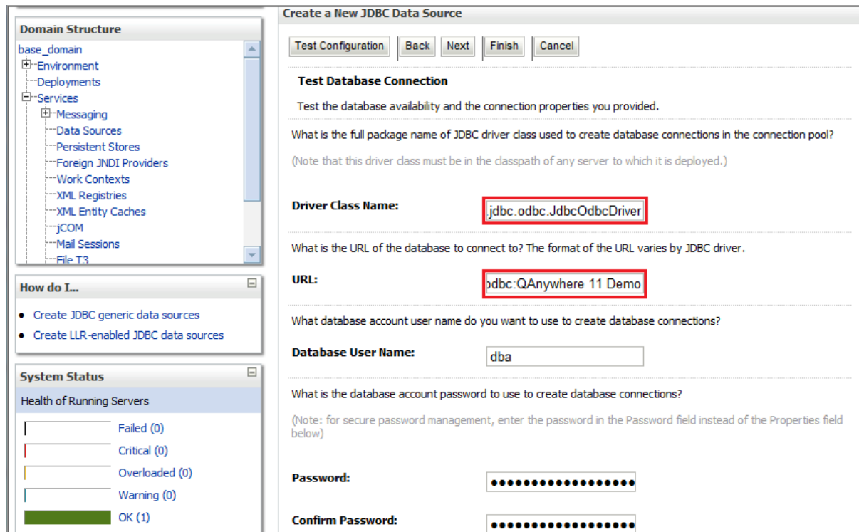
Figure 4.14: Test Database Connection page
