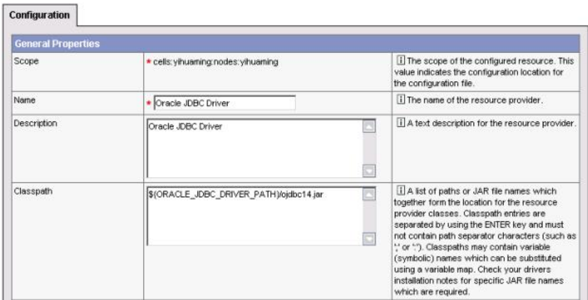
Figure 4.21: JDBC driver provider and driver file
