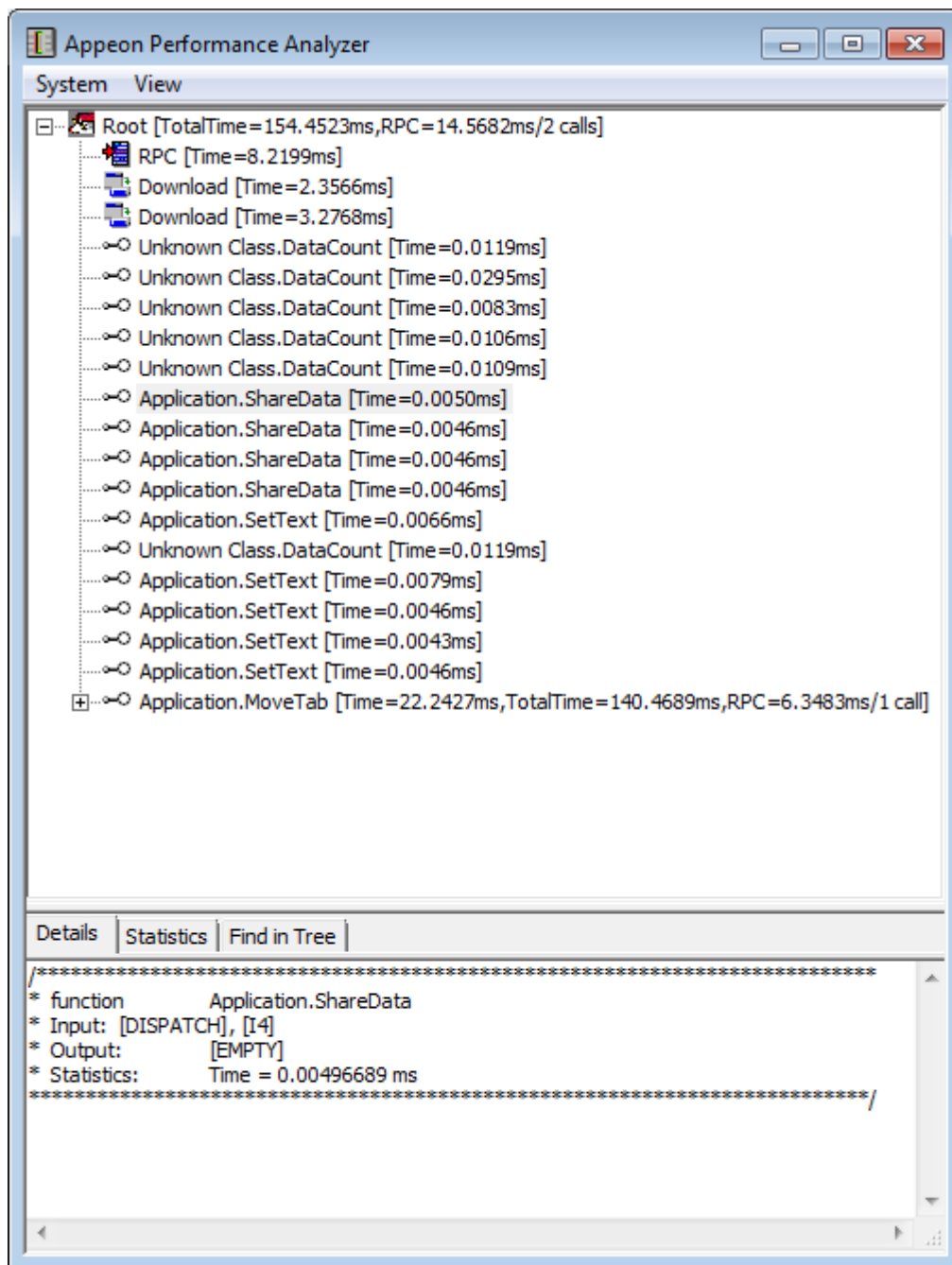
Figure 4.4: Performance analyzer main window
