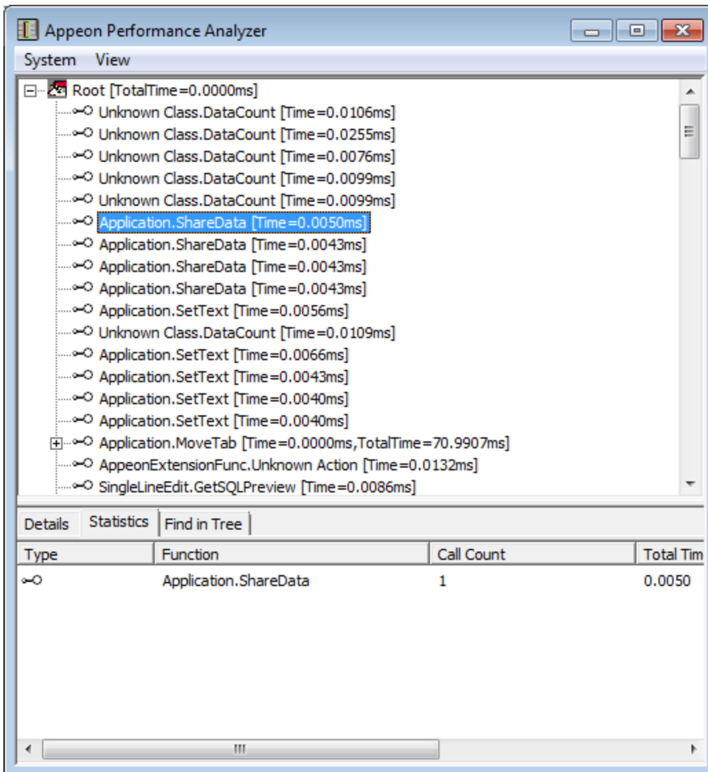
Figure 4.17: View statistics of ActiveX calls
