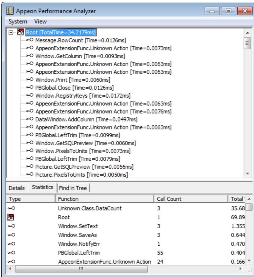
Figure 4.24: View ActiveX calls
