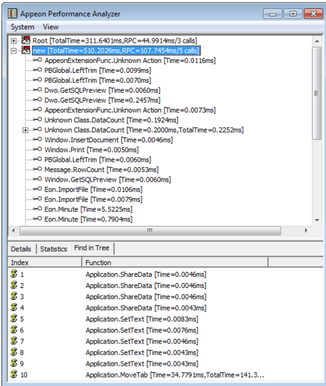
Figure 4.37: Data in the new root item
