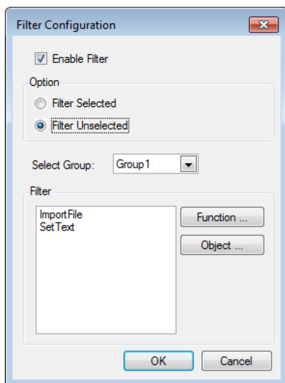
Figure 4.28: Filter Configuration dialog
