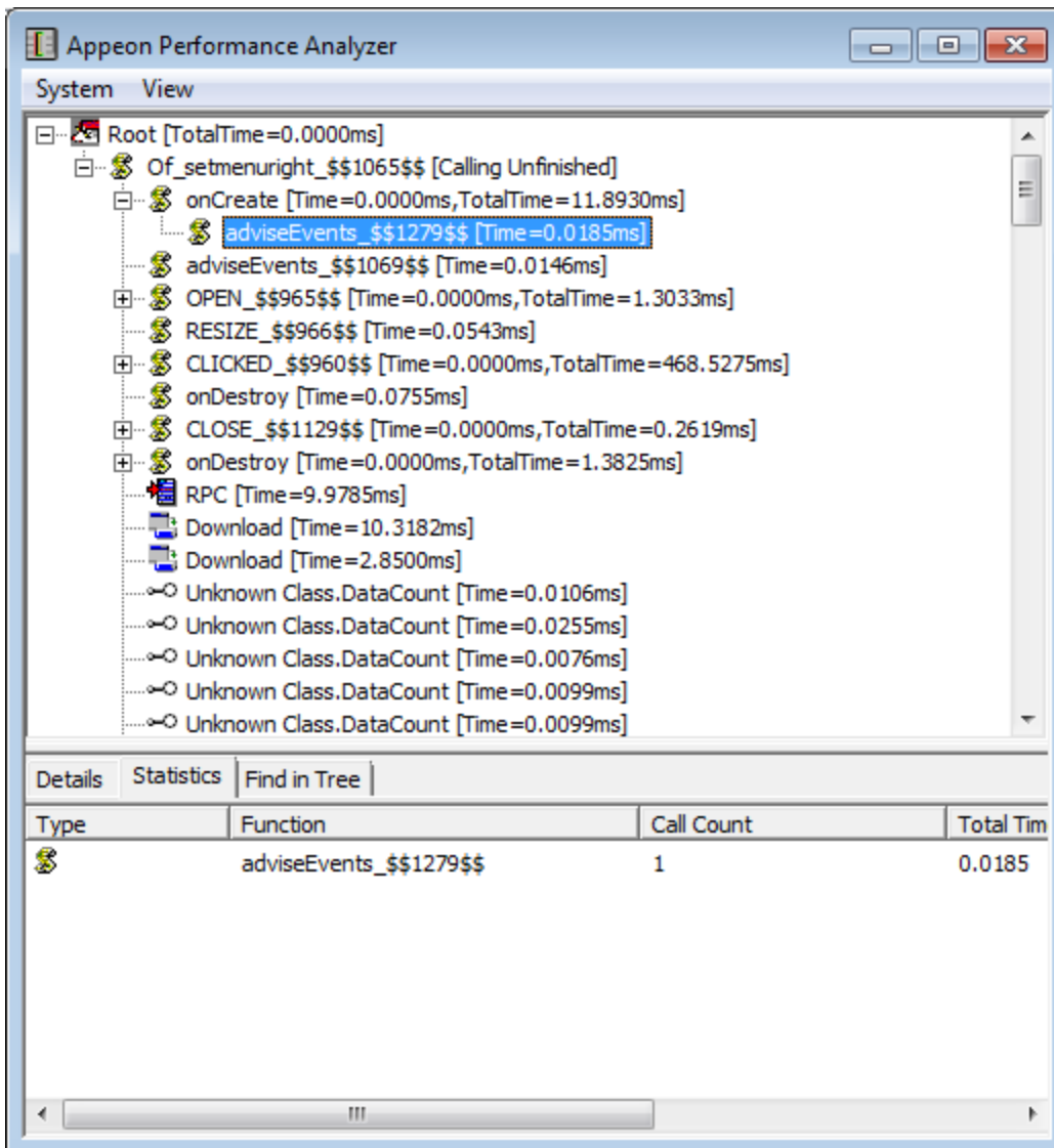
Figure 4.15: View statistics of JavaScript calls
