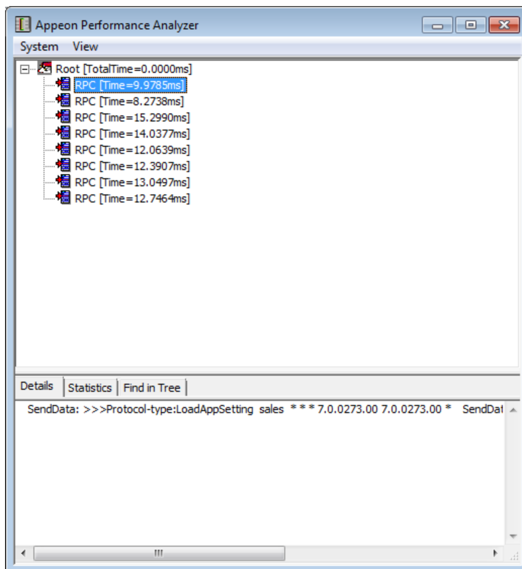
Figure 4.18: View details of RPC calls
