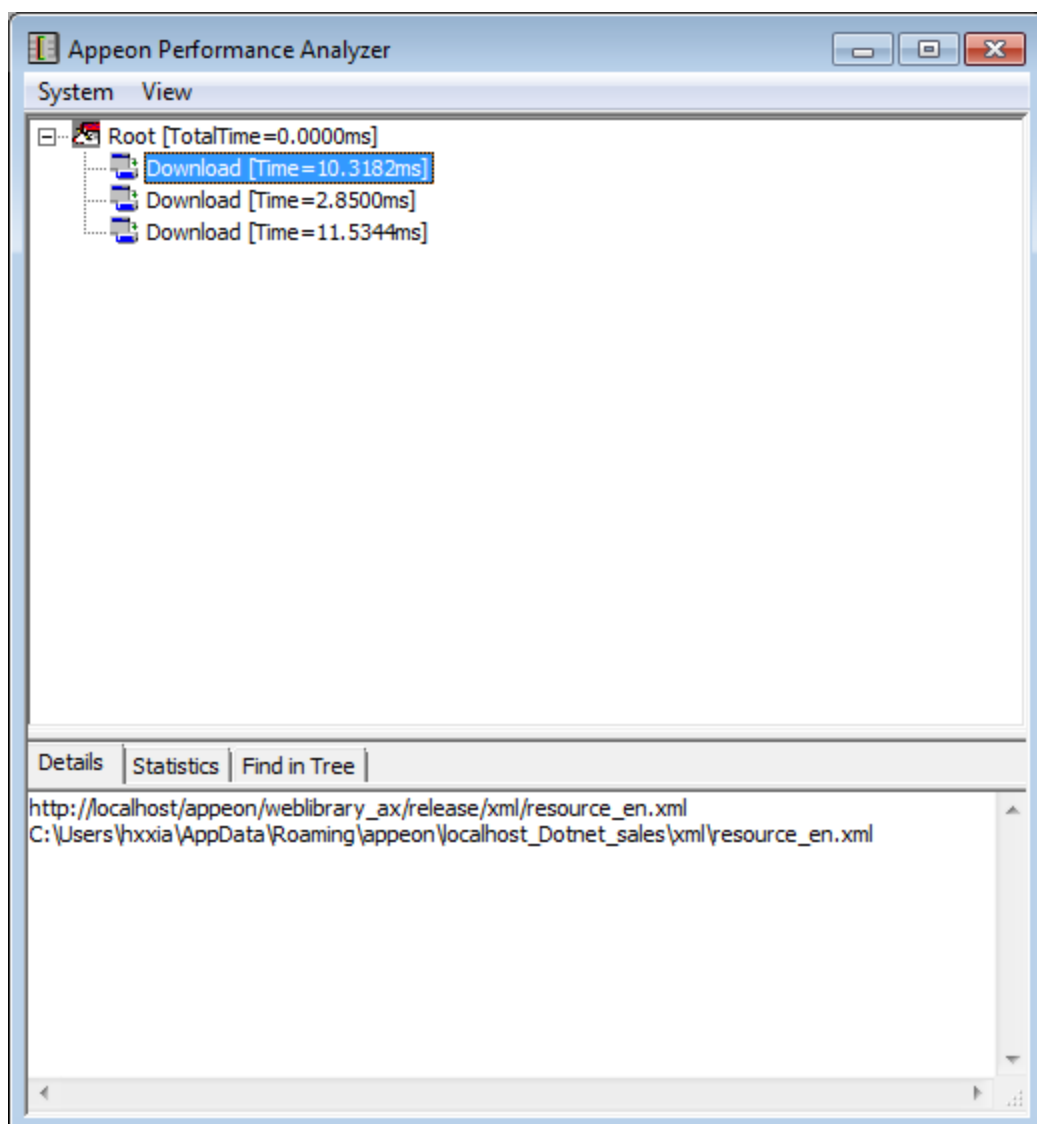
Figure 4.20: View details of downloads
