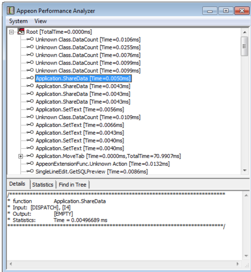
Figure 4.16: View details of ActiveX calls
