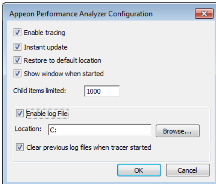
Figure 4.9: Enable log file option
