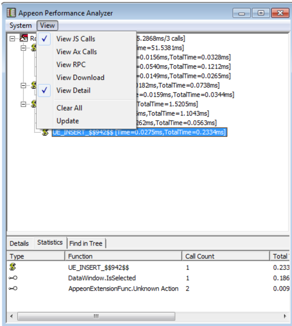
Figure 4.11: View JS Calls menu
