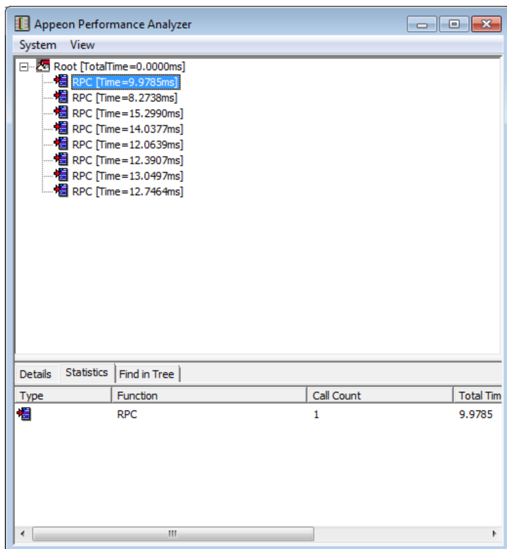
Figure 4.19: View statistics of RPC calls
