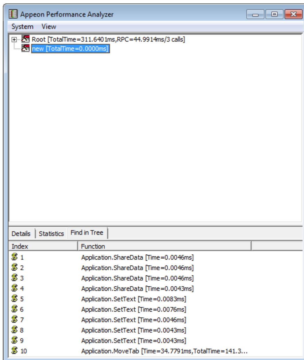
Figure 4.36: New root item is added
