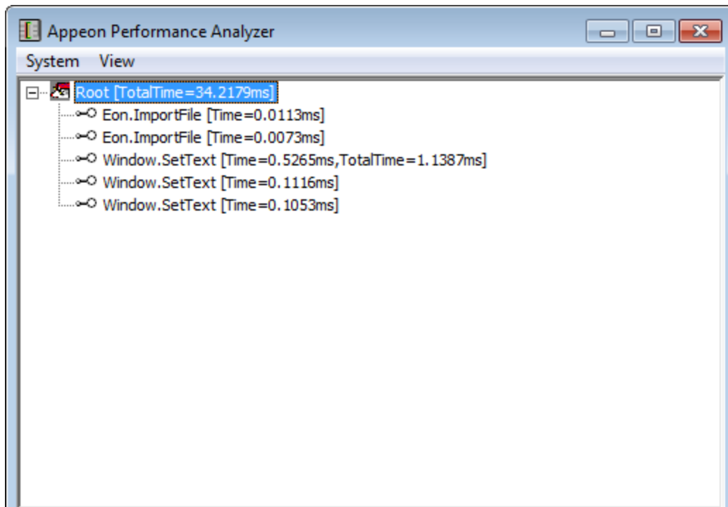
Figure 4.29: Result from Filter Unselected
