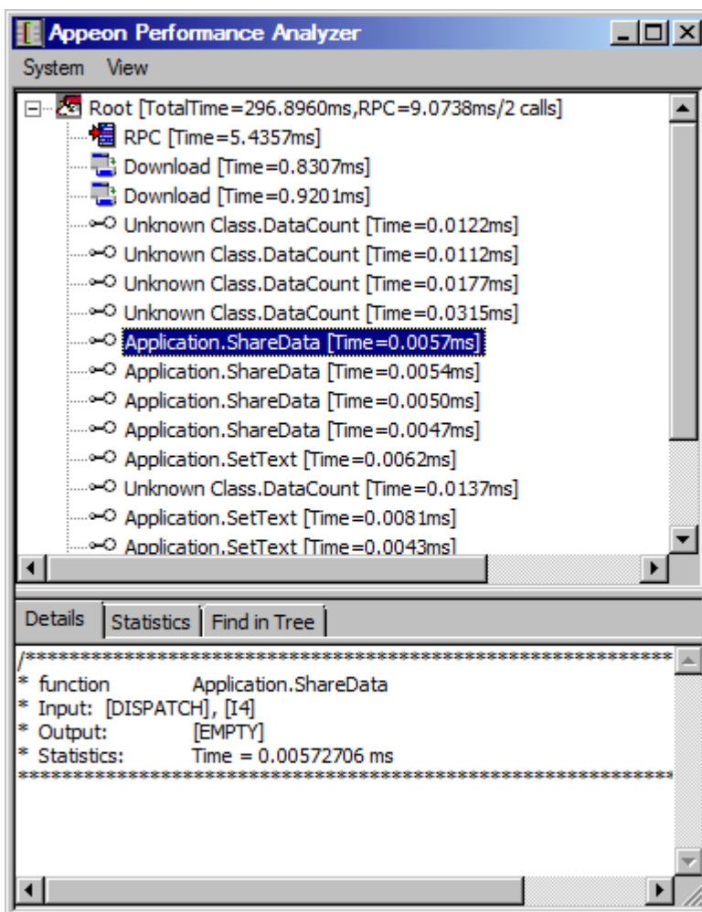
Figure 4.3: Performance analyzer main window
